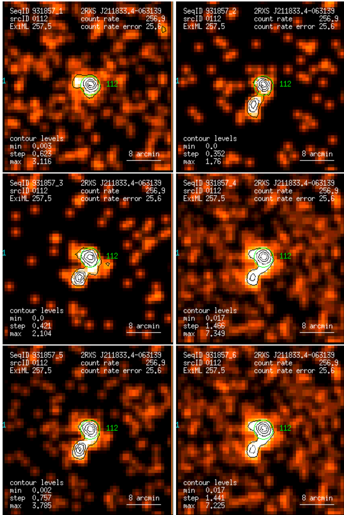
Figure 112: RASS 931857: detection 0112: band rate images, Gaussian filter: (1) PSPC channels 11 – 41, (2) 52 – 90, (3) 91 – 201, (4) 11 – 235, (5) 52 – 201, (6) 11 – 201. Broad band rates in counts/ks. Band rate contour levels in counts/ks/arcmin 2 .
