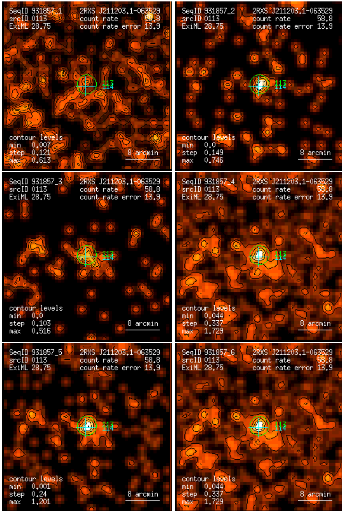
Figure 113: RASS 931857: detection 0113: band rate images, Gaussian filter: (1) PSPC channels 11 – 41, (2) 52 – 90, (3) 91 – 201, (4) 11 – 235, (5) 52 – 201, (6) 11 – 201. Broad band rates in counts/ks. Band rate contour levels in counts/ks/arcmin 2 .
