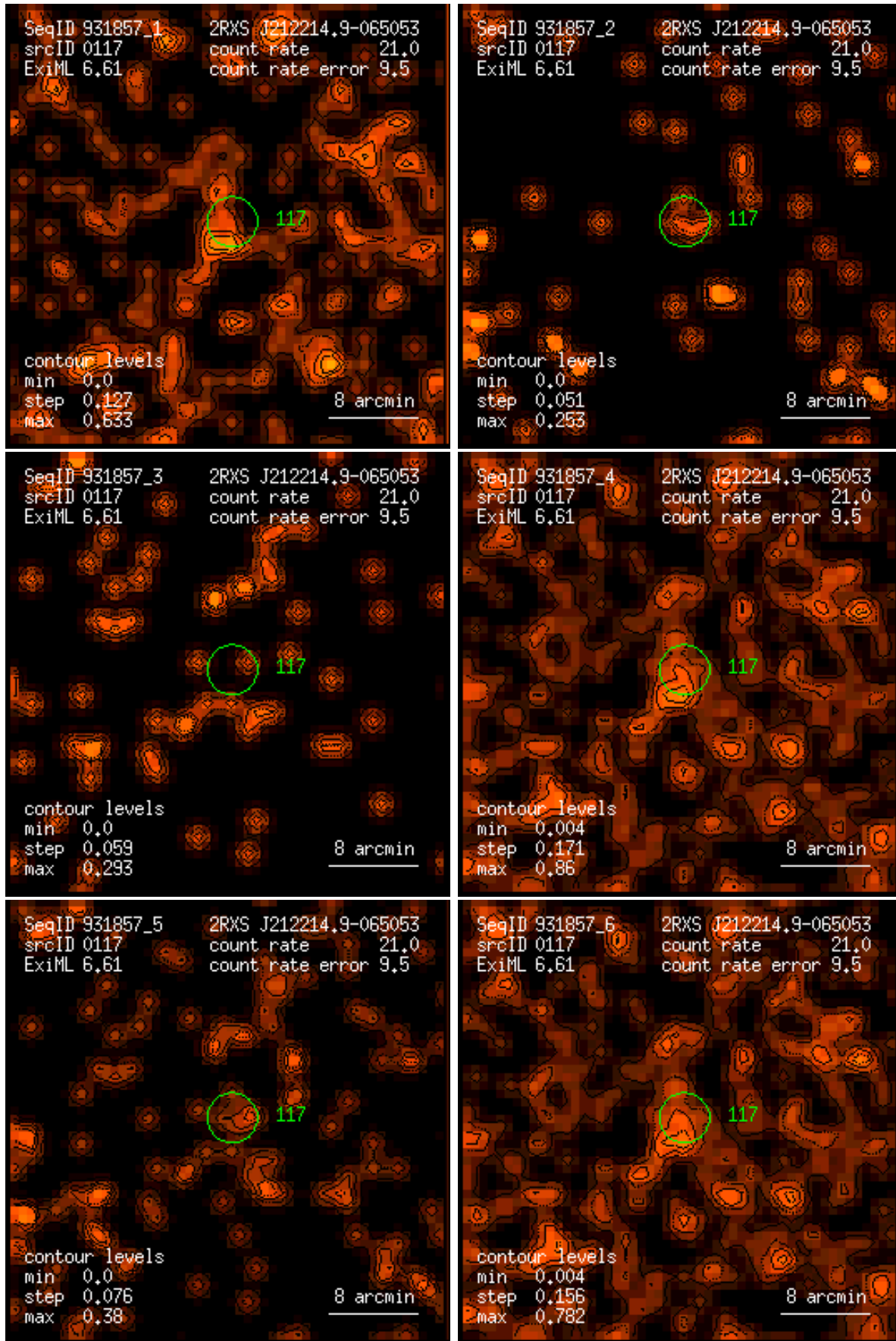
Figure 117: RASS 931857: detection 0117: band rate images, Gaussian filter: (1) PSPC channels 11 – 41, (2) 52 – 90, (3) 91 – 201, (4) 11 – 235, (5) 52 – 201, (6) 11 – 201. Broad band rates in counts/ks. Band rate contour levels in counts/ks/arcmin 2 .
