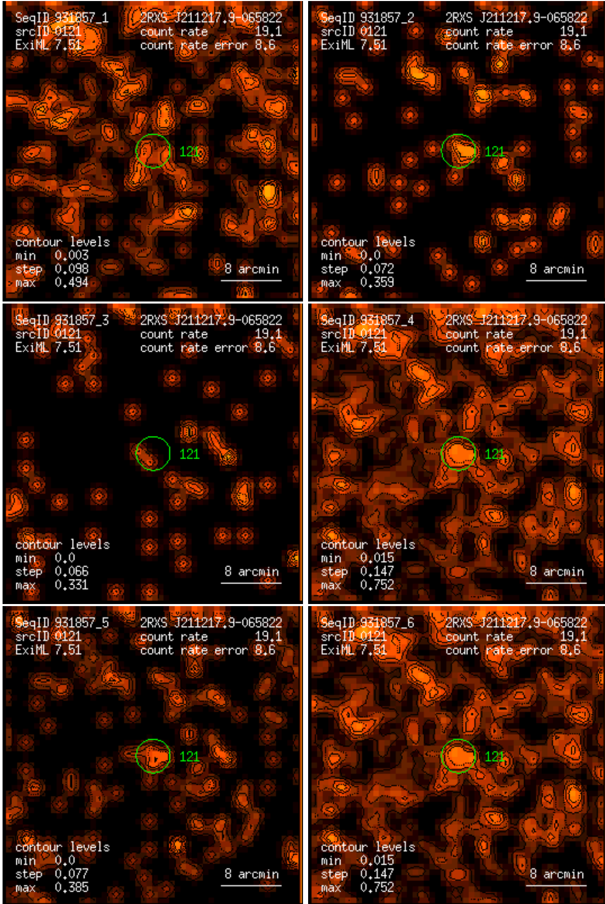
Figure 121: RASS 931857: detection 0121: band rate images, Gaussian filter: (1) PSPC channels 11 – 41, (2) 52 – 90, (3) 91 – 201, (4) 11 – 235, (5) 52 – 201, (6) 11 – 201. Broad band rates in counts/ks. Band rate contour levels in counts/ks/arcmin 2 .
