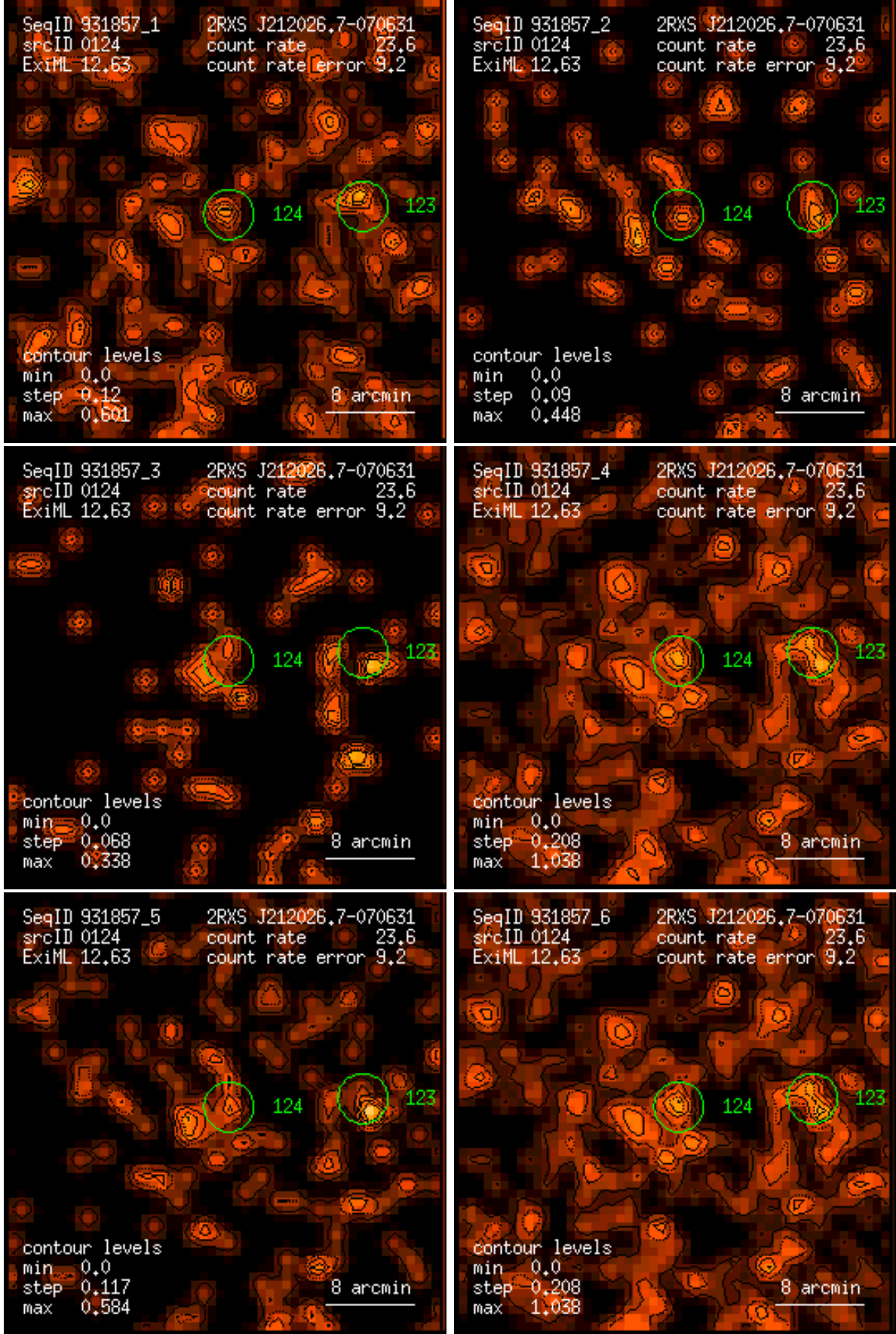
Figure 124: RASS 931857: detection 0124: band rate images, Gaussian filter: (1) PSPC channels 11 – 41, (2) 52 – 90, (3) 91 – 201, (4) 11 – 235, (5) 52 – 201, (6) 11 – 201. Broad band rates in counts/ks. Band rate contour levels in counts/ks/arcmin 2 .
