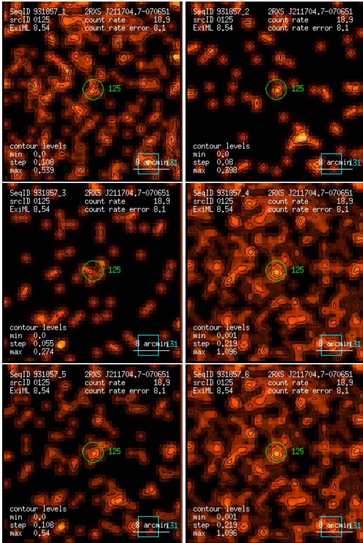
Figure 125: RASS 931857: detection 0125: band rate images, Gaussian filter: (1) PSPC channels 11 – 41, (2) 52 – 90, (3) 91 – 201, (4) 11 – 235, (5) 52 – 201, (6) 11 – 201. Broad band rates in counts/ks. Band rate contour levels in counts/ks/arcmin 2 .
