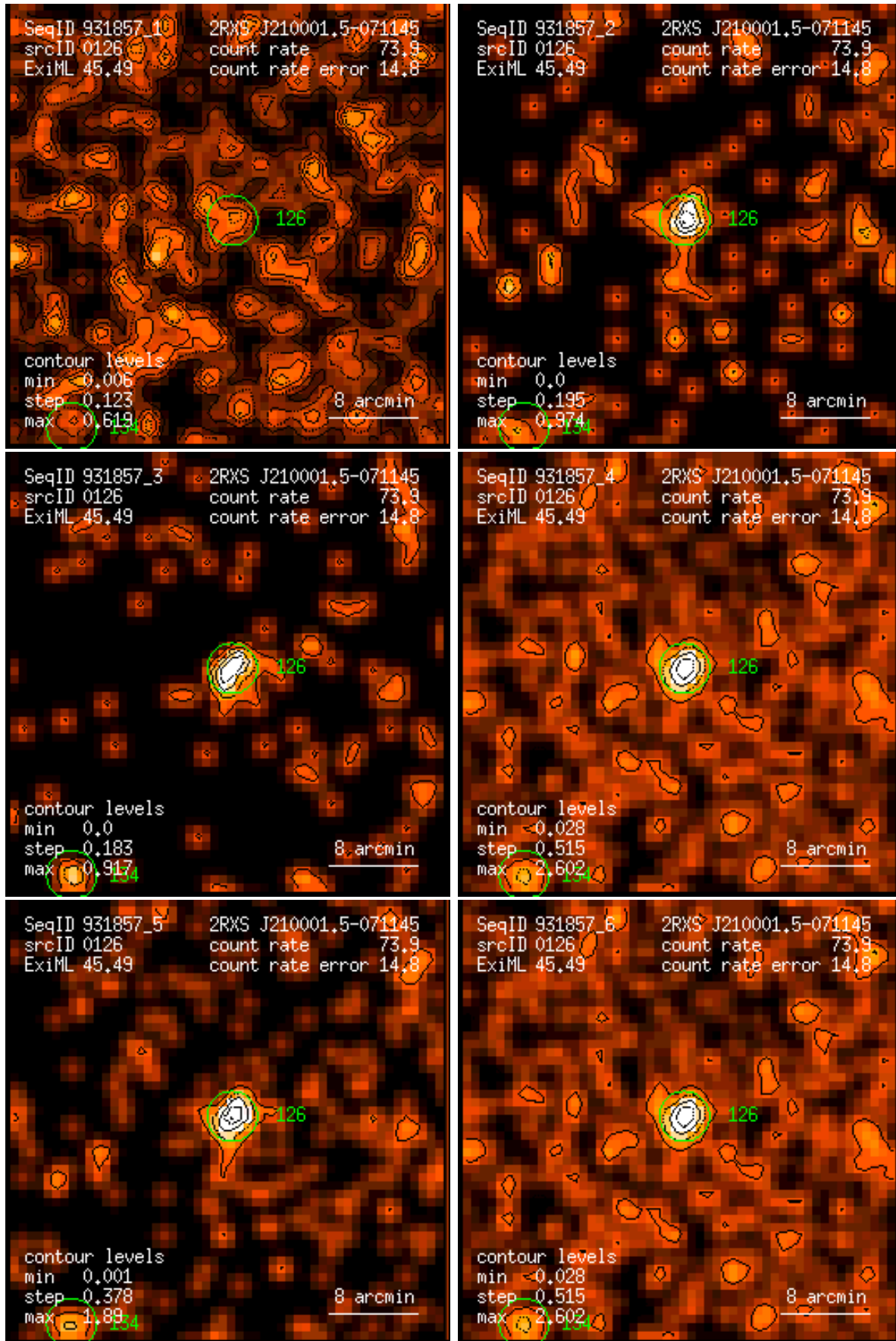
Figure 126: RASS 931857: detection 0126: band rate images, Gaussian filter: (1) PSPC channels 11 – 41, (2) 52 – 90, (3) 91 – 201, (4) 11 – 235, (5) 52 – 201, (6) 11 – 201. Broad band rates in counts/ks. Band rate contour levels in counts/ks/arcmin 2 .
