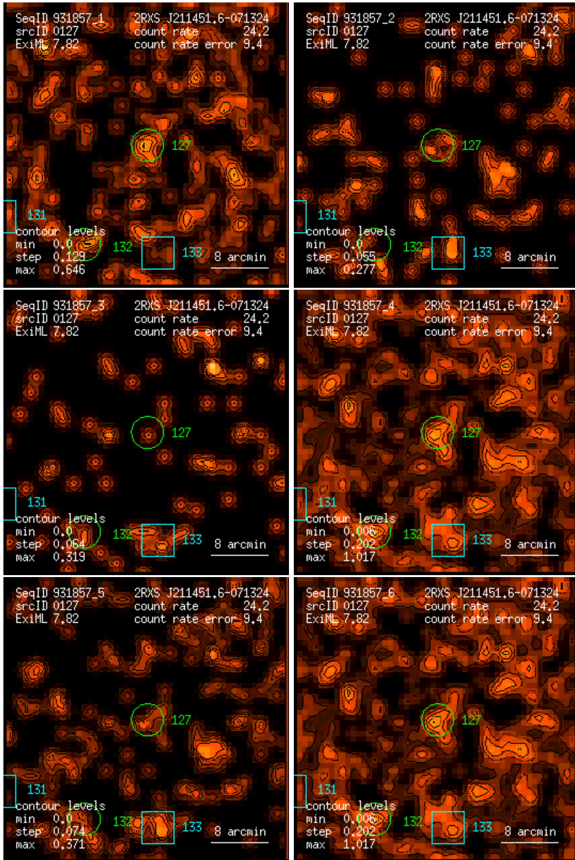
Figure 127: RASS 931857: detection 0127: band rate images, Gaussian filter: (1) PSPC channels 11 – 41, (2) 52 – 90, (3) 91 – 201, (4) 11 – 235, (5) 52 – 201, (6) 11 – 201. Broad band rates in counts/ks. Band rate contour levels in counts/ks/arcmin 2 .
