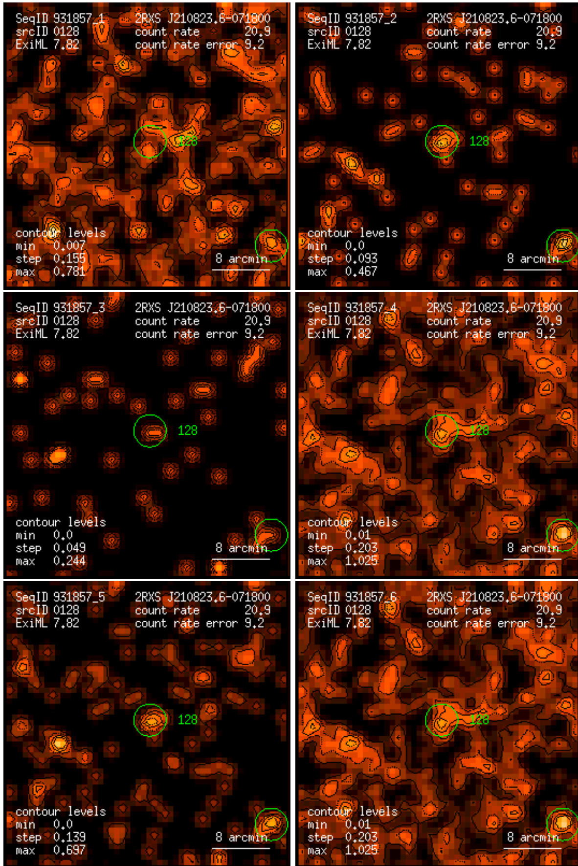
Figure 128: RASS 931857: detection 0128: band rate images, Gaussian filter: (1) PSPC channels 11 – 41, (2) 52 – 90, (3) 91 – 201, (4) 11 – 235, (5) 52 – 201, (6) 11 – 201. Broad band rates in counts/ks. Band rate contour levels in counts/ks/arcmin 2 .
