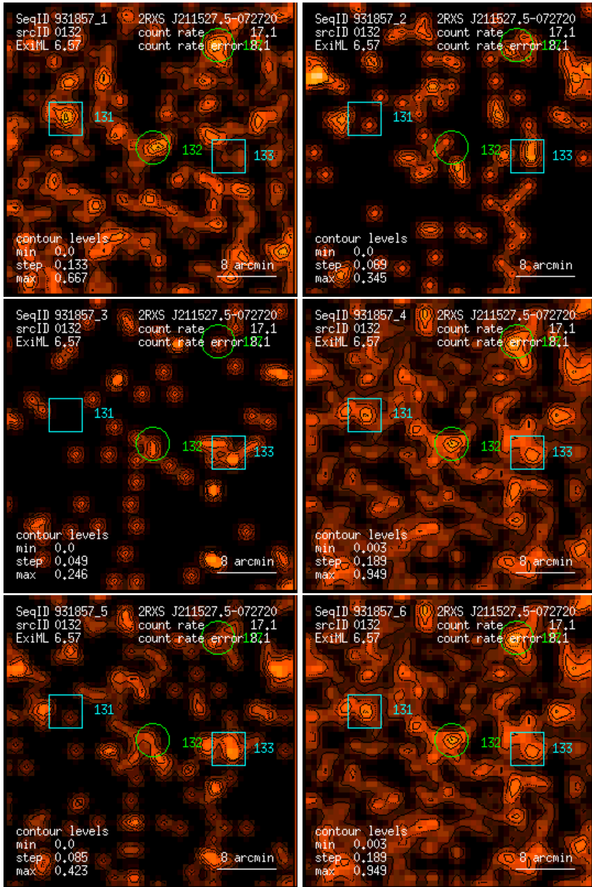
Figure 132: RASS 931857: detection 0132: band rate images, Gaussian filter: (1) PSPC channels 11 – 41, (2) 52 – 90, (3) 91 – 201, (4) 11 – 235, (5) 52 – 201, (6) 11 – 201. Broad band rates in counts/ks. Band rate contour levels in counts/ks/arcmin 2 .
