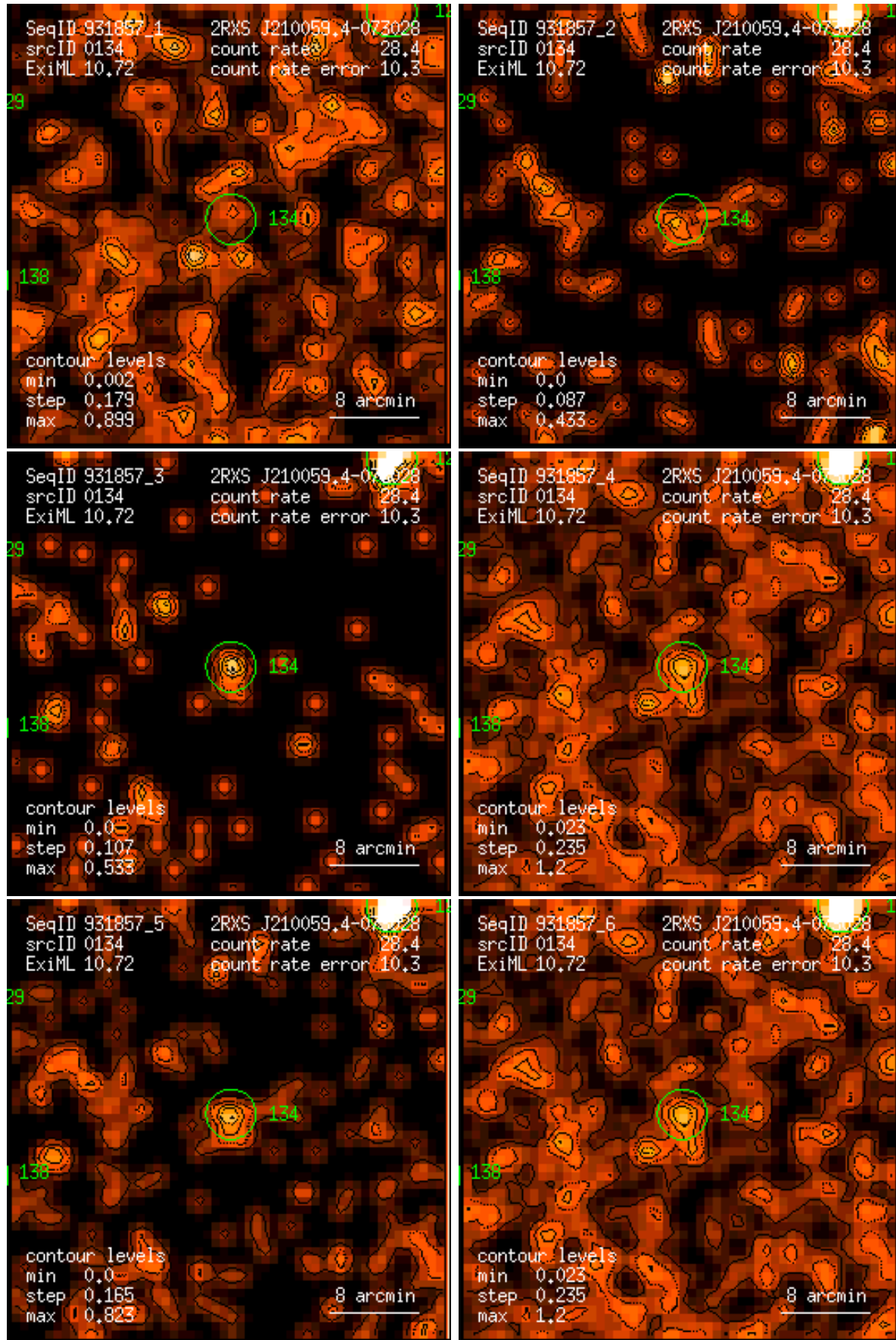
Figure 134: RASS 931857: detection 0134: band rate images, Gaussian filter: (1) PSPC channels 11 – 41, (2) 52 – 90, (3) 91 – 201, (4) 11 – 235, (5) 52 – 201, (6) 11 – 201. Broad band rates in counts/ks. Band rate contour levels in counts/ks/arcmin 2 .
