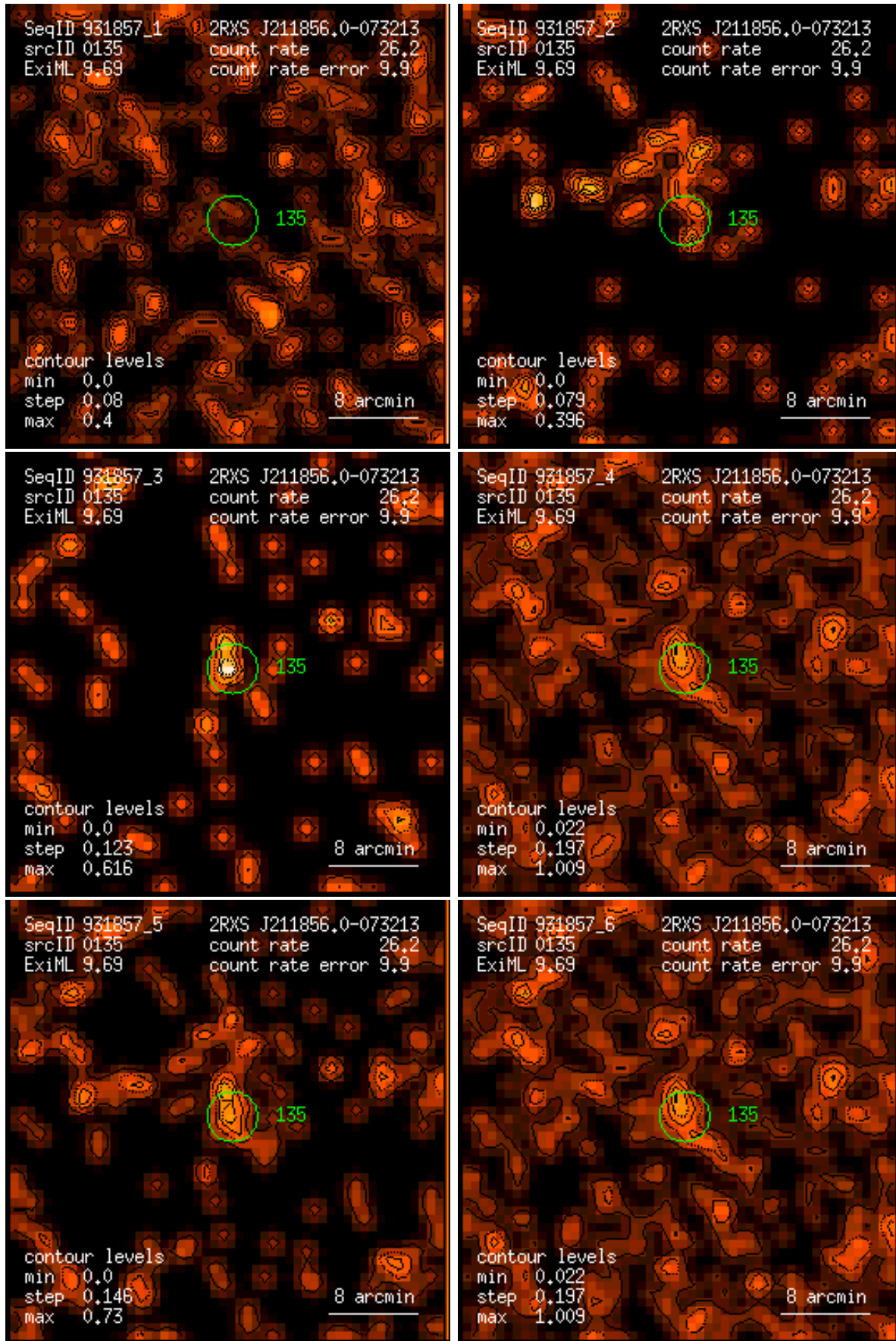
Figure 135: RASS 931857: detection 0135: band rate images, Gaussian filter: (1) PSPC channels 11 – 41, (2) 52 – 90, (3) 91 – 201, (4) 11 – 235, (5) 52 – 201, (6) 11 – 201. Broad band rates in counts/ks. Band rate contour levels in counts/ks/arcmin 2 .
