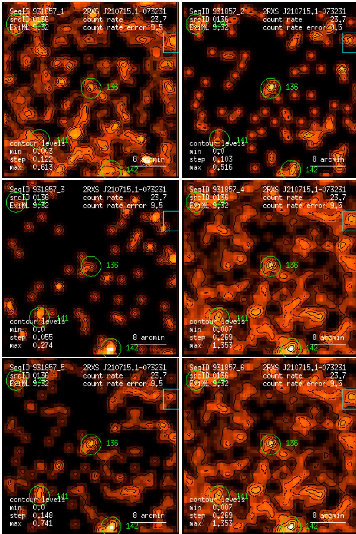
Figure 136: RASS 931857: detection 0136: band rate images, Gaussian filter: (1) PSPC channels 11 – 41, (2) 52 – 90, (3) 91 – 201, (4) 11 – 235, (5) 52 – 201, (6) 11 – 201. Broad band rates in counts/ks. Band rate contour levels in counts/ks/arcmin 2 .
