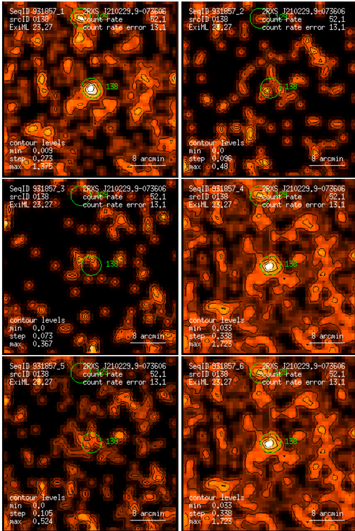
Figure 138: RASS 931857: detection 0138: band rate images, Gaussian filter: (1) PSPC channels 11 – 41, (2) 52 – 90, (3) 91 – 201, (4) 11 – 235, (5) 52 – 201, (6) 11 – 201. Broad band rates in counts/ks. Band rate contour levels in counts/ks/arcmin 2 .
