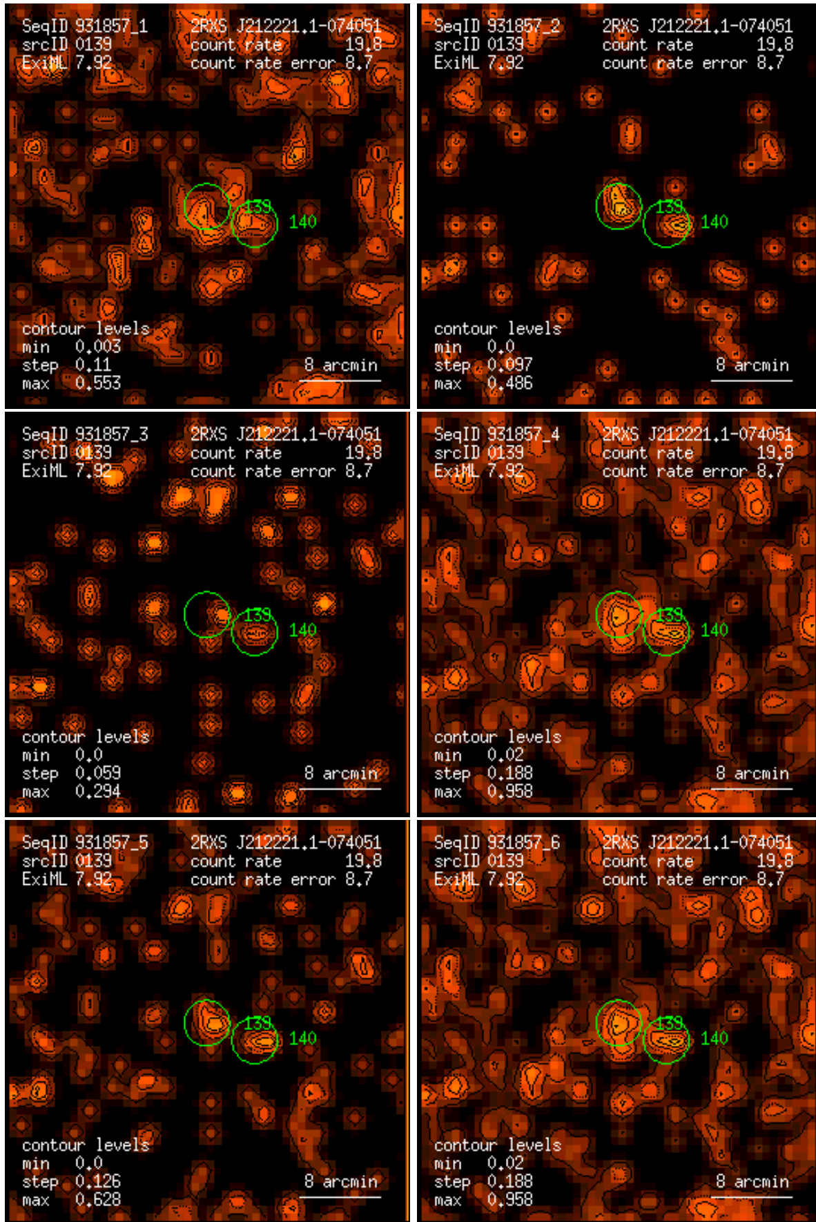
Figure 139: RASS 931857: detection 0139: band rate images, Gaussian filter: (1) PSPC channels 11 – 41, (2) 52 – 90, (3) 91 – 201, (4) 11 – 235, (5) 52 – 201, (6) 11 – 201. Broad band rates in counts/ks. Band rate contour levels in counts/ks/arcmin 2 .
