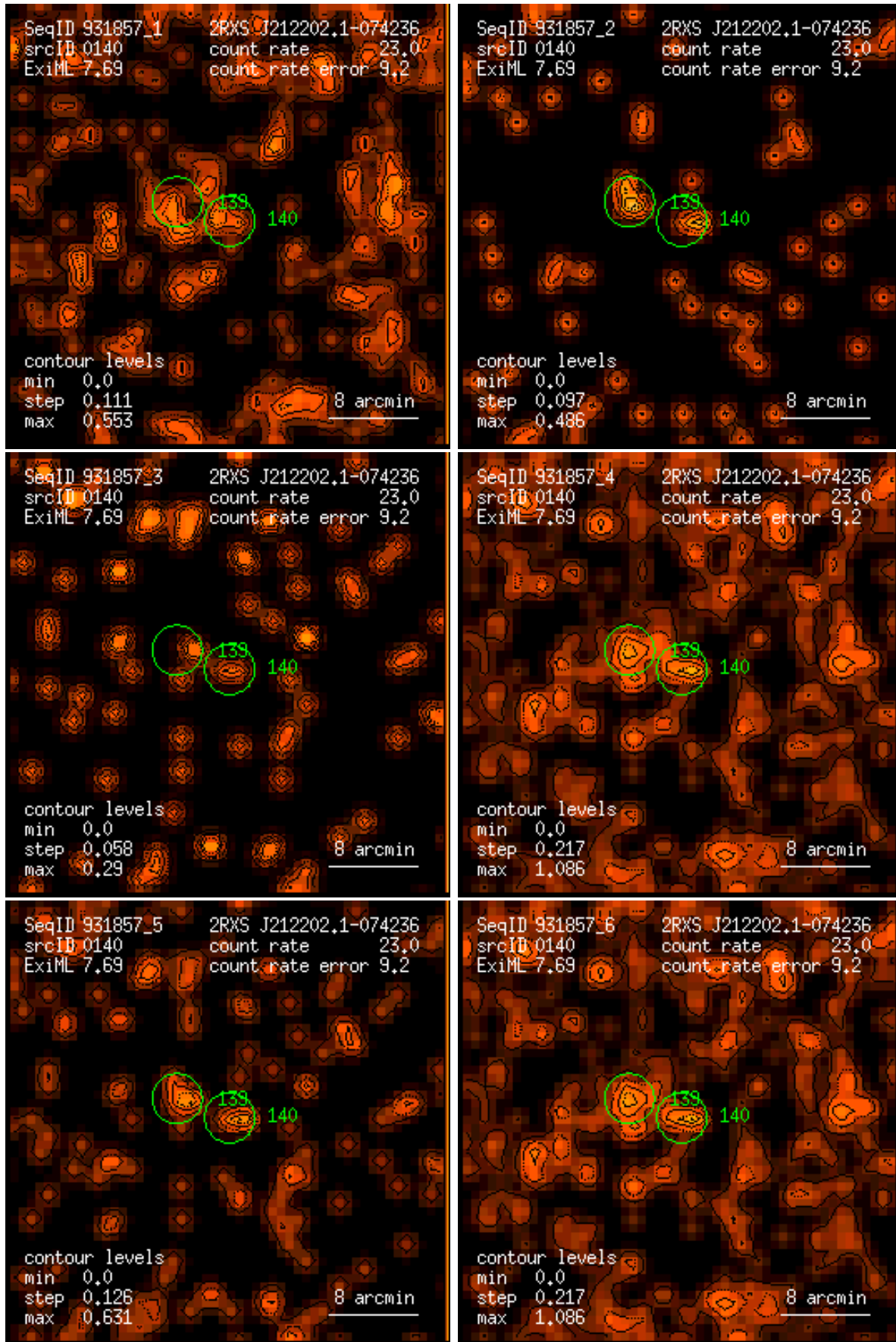
Figure 140: RASS 931857: detection 0140: band rate images, Gaussian filter: (1) PSPC channels 11 – 41, (2) 52 – 90, (3) 91 – 201, (4) 11 – 235, (5) 52 – 201, (6) 11 – 201. Broad band rates in counts/ks. Band rate contour levels in counts/ks/arcmin 2 .
