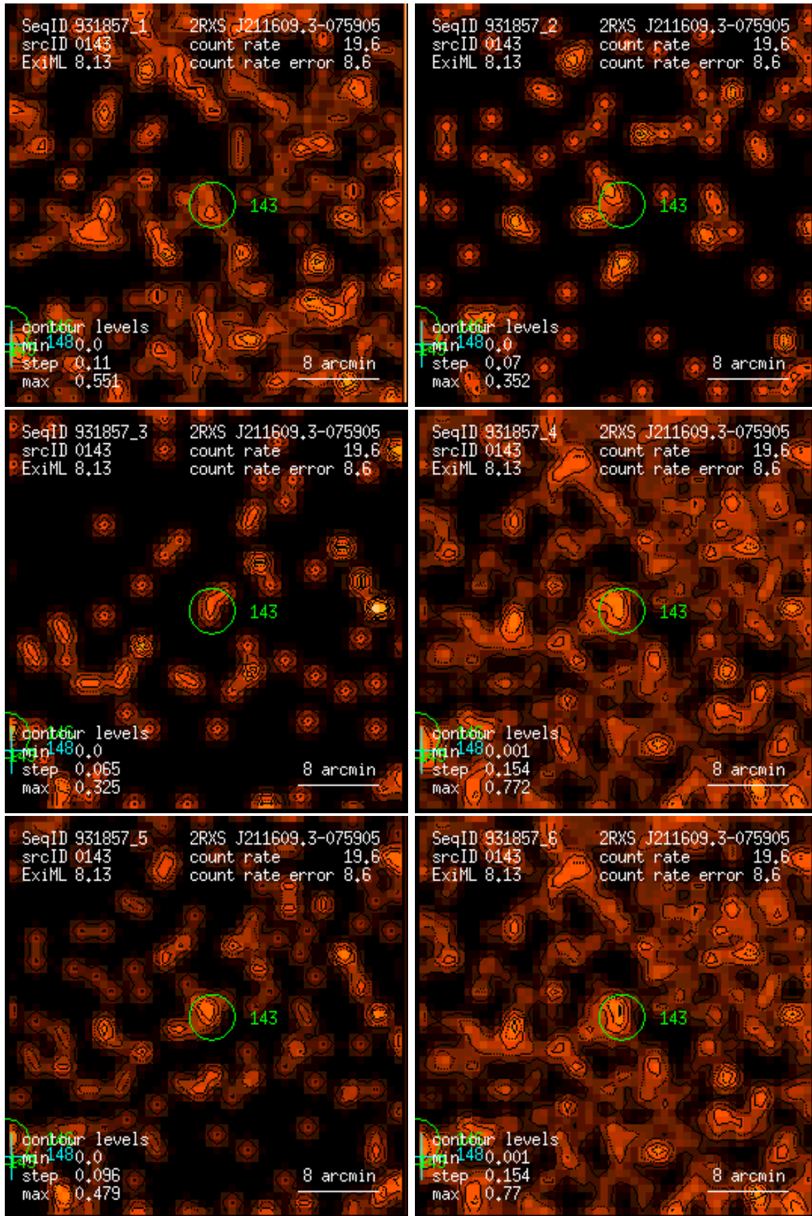
Figure 143: RASS 931857: detection 0143: band rate images, Gaussian filter: (1) PSPC channels 11 – 41, (2) 52 – 90, (3) 91 – 201, (4) 11 – 235, (5) 52 – 201, (6) 11 – 201. Broad band rates in counts/ks. Band rate contour levels in counts/ks/arcmin 2 .
