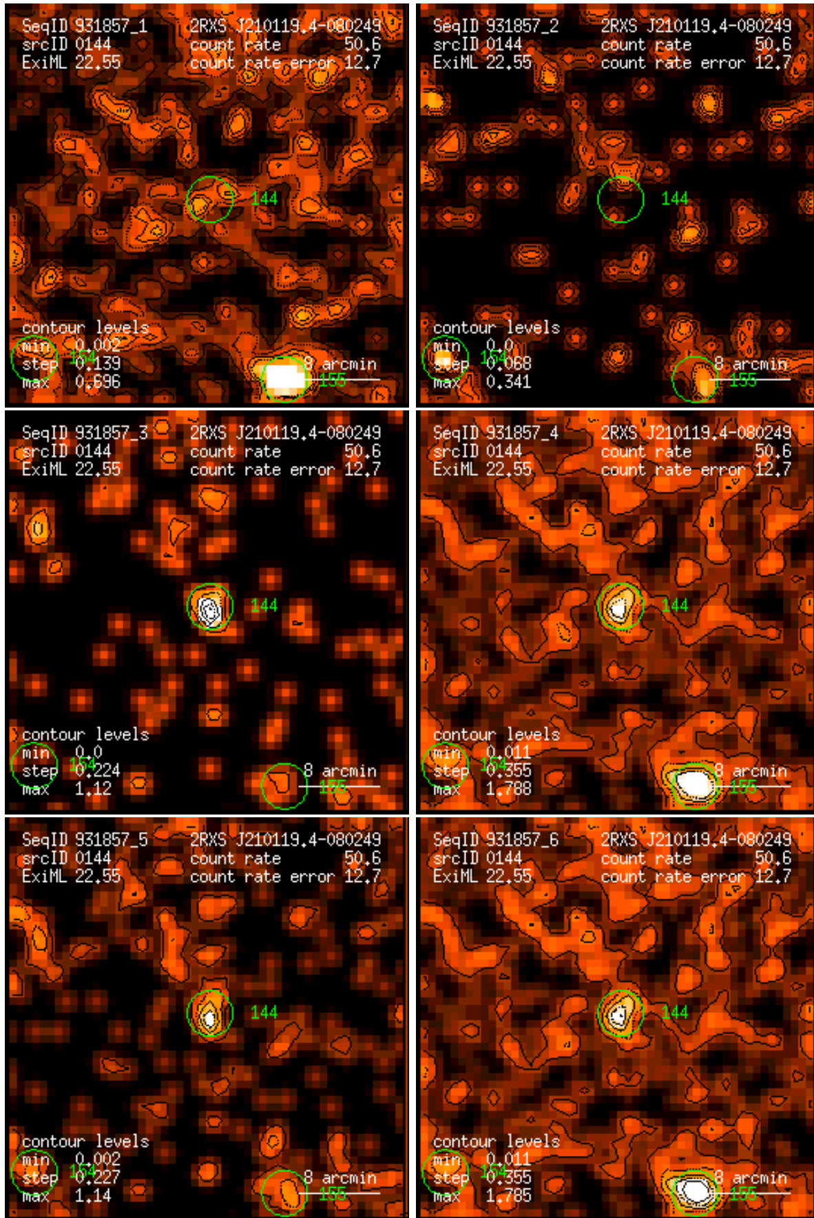
Figure 144: RASS 931857: detection 0144: band rate images, Gaussian filter: (1) PSPC channels 11 – 41, (2) 52 – 90, (3) 91 – 201, (4) 11 – 235, (5) 52 – 201, (6) 11 – 201. Broad band rates in counts/ks. Band rate contour levels in counts/ks/arcmin 2 .
