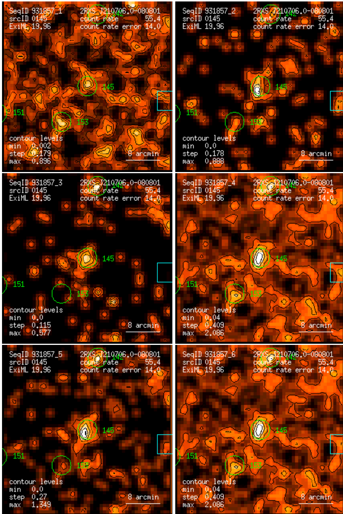
Figure 145: RASS 931857: detection 0145: band rate images, Gaussian filter: (1) PSPC channels 11 – 41, (2) 52 – 90, (3) 91 – 201, (4) 11 – 235, (5) 52 – 201, (6) 11 – 201. Broad band rates in counts/ks. Band rate contour levels in counts/ks/arcmin 2 .
