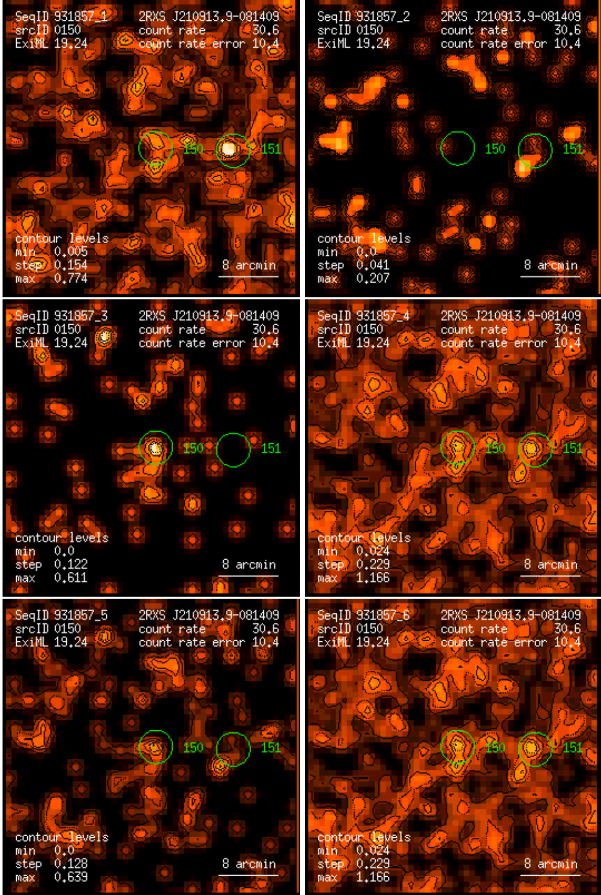
Figure 150: RASS 931857: detection 0150: band rate images, Gaussian filter: (1) PSPC channels 11 – 41, (2) 52 – 90, (3) 91 – 201, (4) 11 – 235, (5) 52 – 201, (6) 11 – 201. Broad band rates in counts/ks. Band rate contour levels in counts/ks/arcmin 2 .
