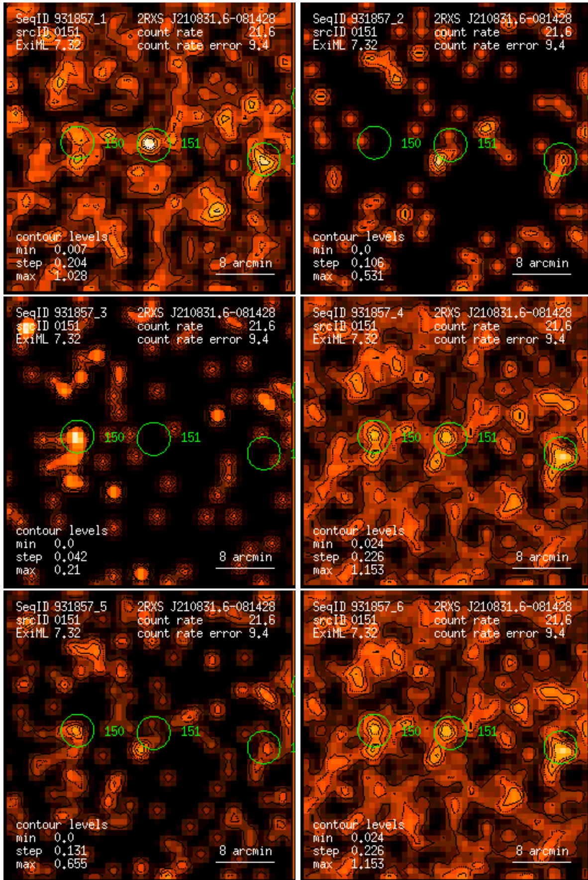
Figure 151: RASS 931857: detection 0151: band rate images, Gaussian filter: (1) PSPC channels 11 – 41, (2) 52 – 90, (3) 91 – 201, (4) 11 – 235, (5) 52 – 201, (6) 11 – 201. Broad band rates in counts/ks. Band rate contour levels in counts/ks/arcmin 2 .
