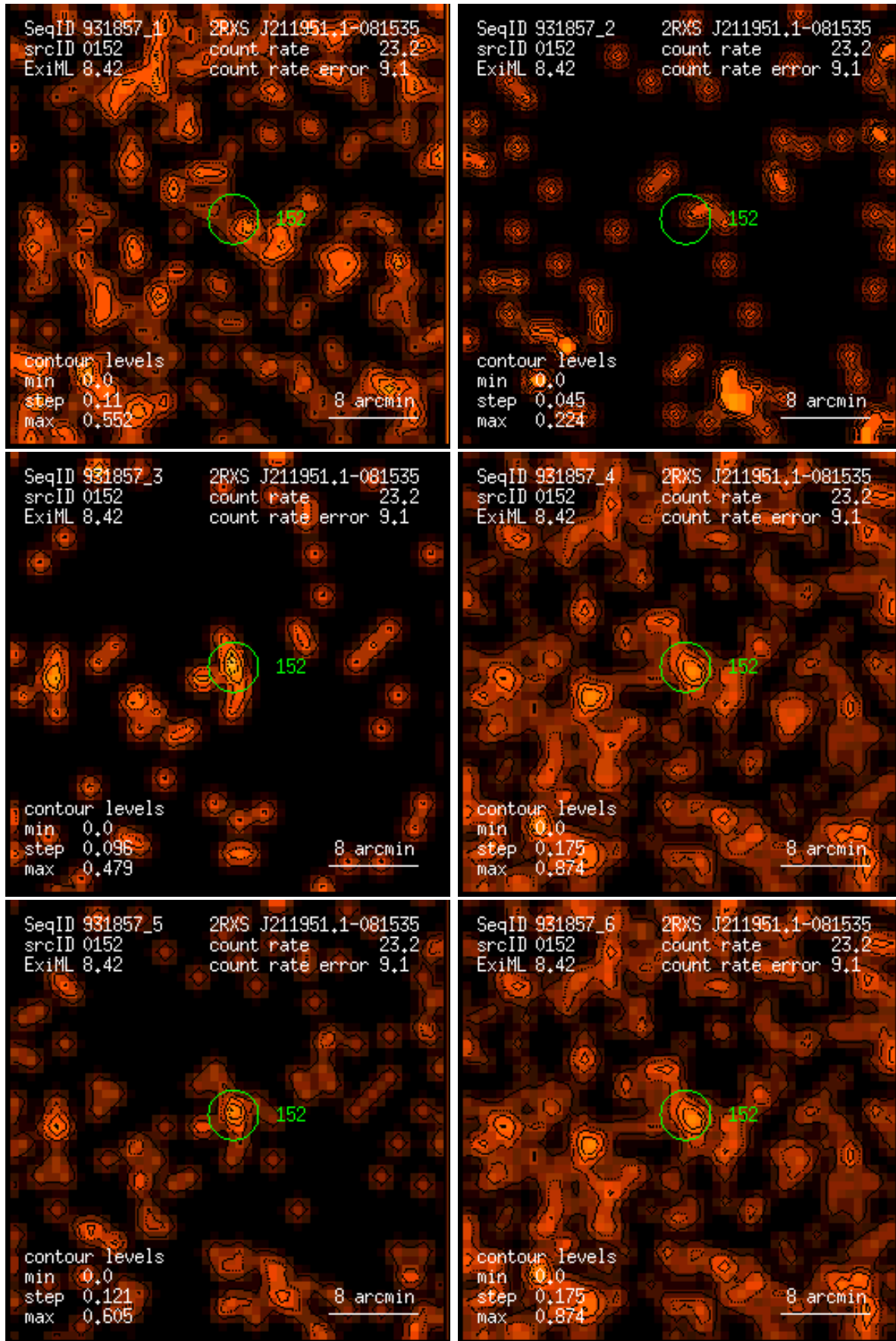
Figure 152: RASS 931857: detection 0152: band rate images, Gaussian filter: (1) PSPC channels 11 – 41, (2) 52 – 90, (3) 91 – 201, (4) 11 – 235, (5) 52 – 201, (6) 11 – 201. Broad band rates in counts/ks. Band rate contour levels in counts/ks/arcmin 2 .
