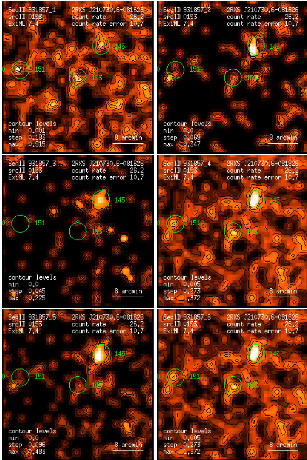
Figure 153: RASS 931857: detection 0153: band rate images, Gaussian filter: (1) PSPC channels 11 – 41, (2) 52 – 90, (3) 91 – 201, (4) 11 – 235, (5) 52 – 201, (6) 11 – 201. Broad band rates in counts/ks. Band rate contour levels in counts/ks/arcmin 2 .
