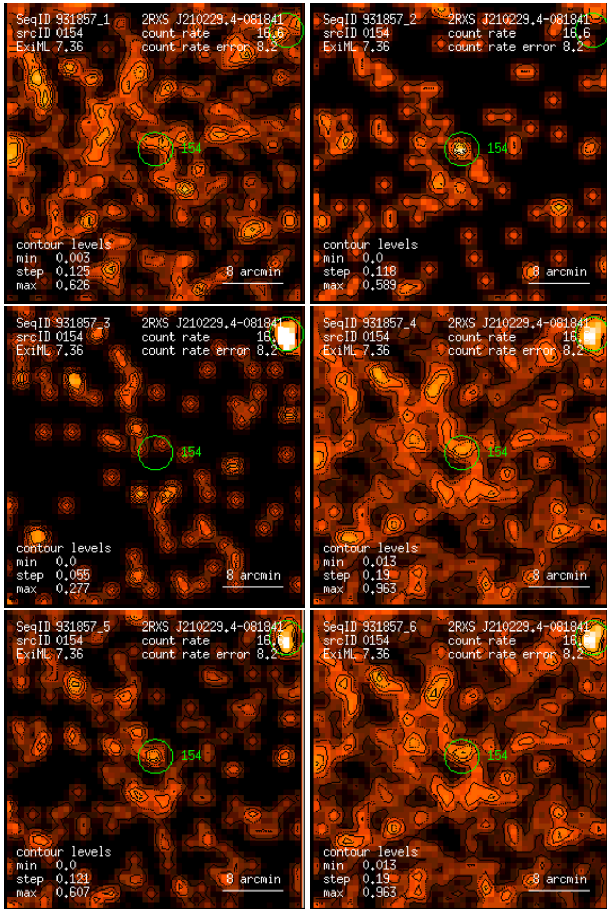
Figure 154: RASS 931857: detection 0154: band rate images, Gaussian filter: (1) PSPC channels 11 – 41, (2) 52 – 90, (3) 91 – 201, (4) 11 – 235, (5) 52 – 201, (6) 11 – 201. Broad band rates in counts/ks. Band rate contour levels in counts/ks/arcmin 2 .
