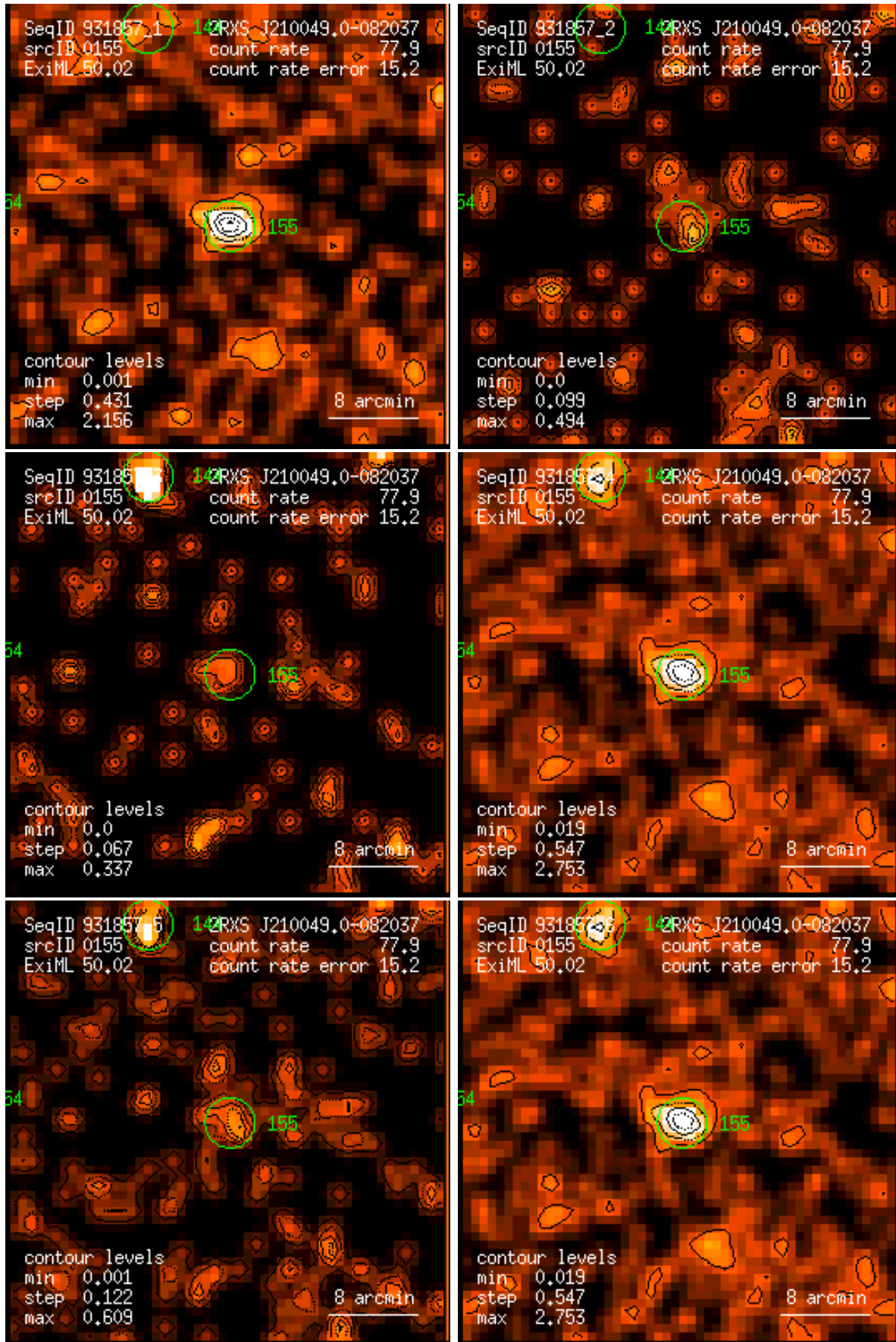
Figure 155: RASS 931857: detection 0155: band rate images, Gaussian filter: (1) PSPC channels 11 – 41, (2) 52 – 90, (3) 91 – 201, (4) 11 – 235, (5) 52 – 201, (6) 11 – 201. Broad band rates in counts/ks. Band rate contour levels in counts/ks/arcmin 2 .
