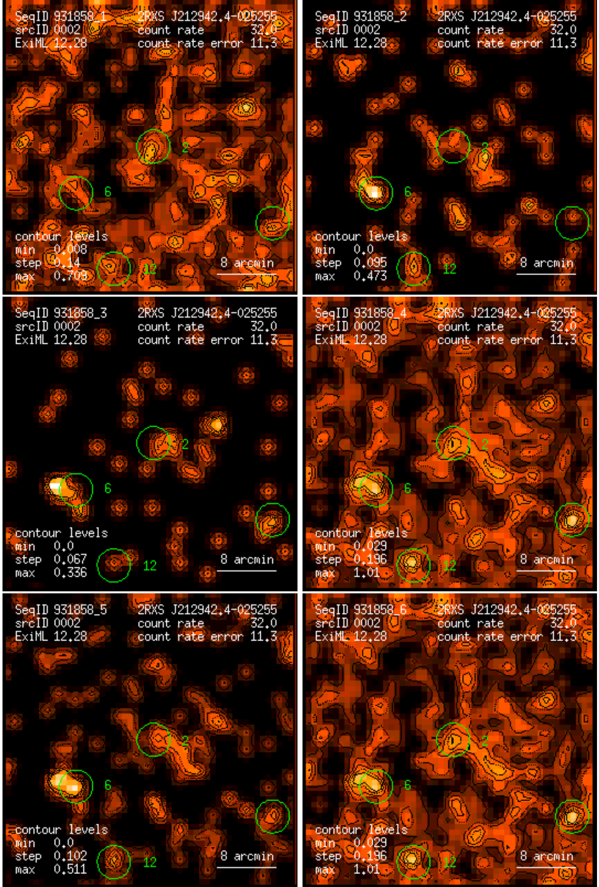
Figure 2: RASS 931858: detection 0002: band rate images, Gaussian filter: (1) PSPC channels 11 – 41, (2) 52 – 90, (3) 91 – 201, (4) 11 – 235, (5) 52 – 201, (6) 11 – 201. Broad band rates in counts/ks. Band rate contour levels in counts/ks/arcmin 2 .
