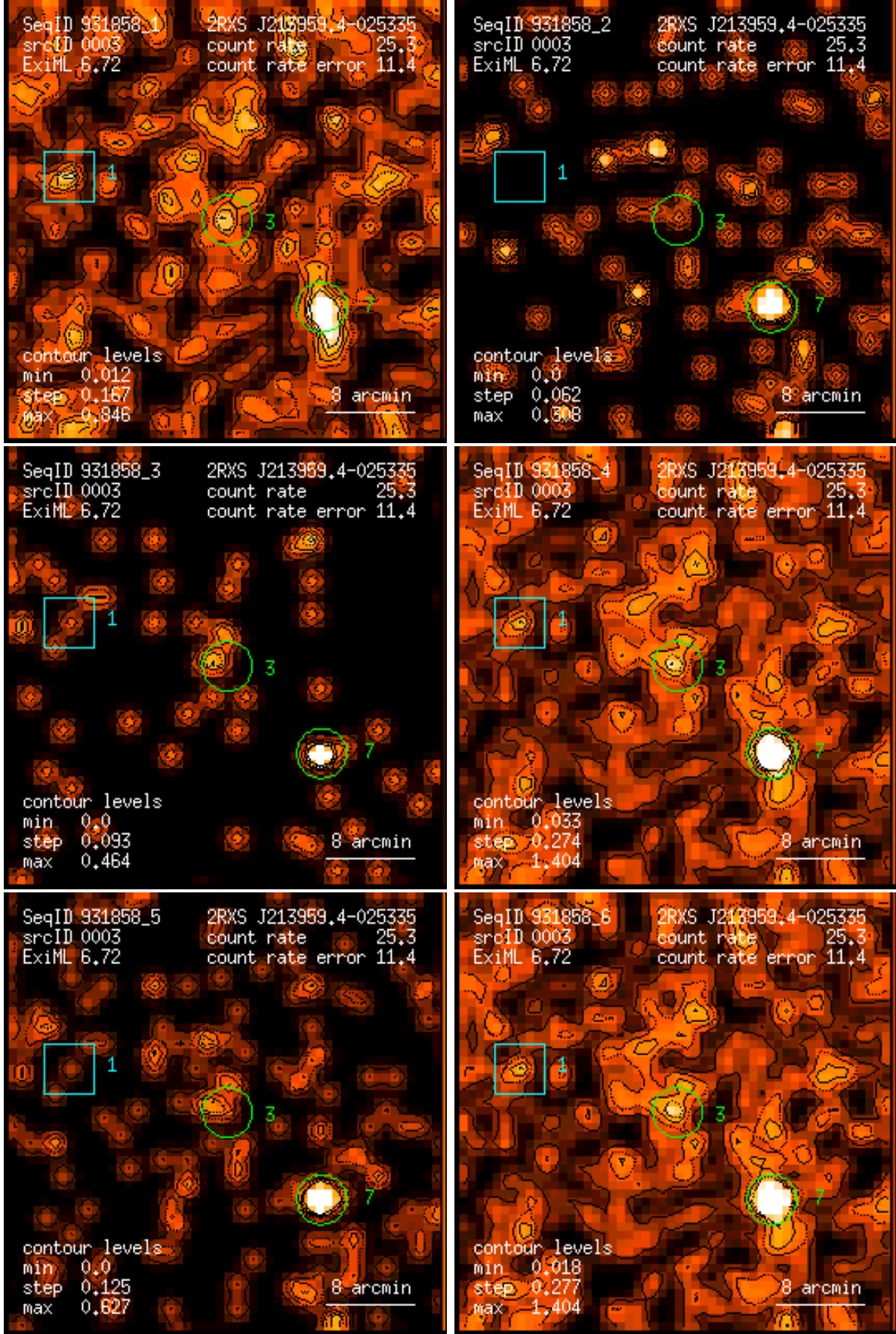
Figure 3: RASS 931858: detection 0003: band rate images, Gaussian filter: (1) PSPC channels 11 – 41, (2) 52 – 90, (3) 91 – 201, (4) 11 – 235, (5) 52 – 201, (6) 11 – 201. Broad band rates in counts/ks. Band rate contour levels in counts/ks/arcmin 2 .
