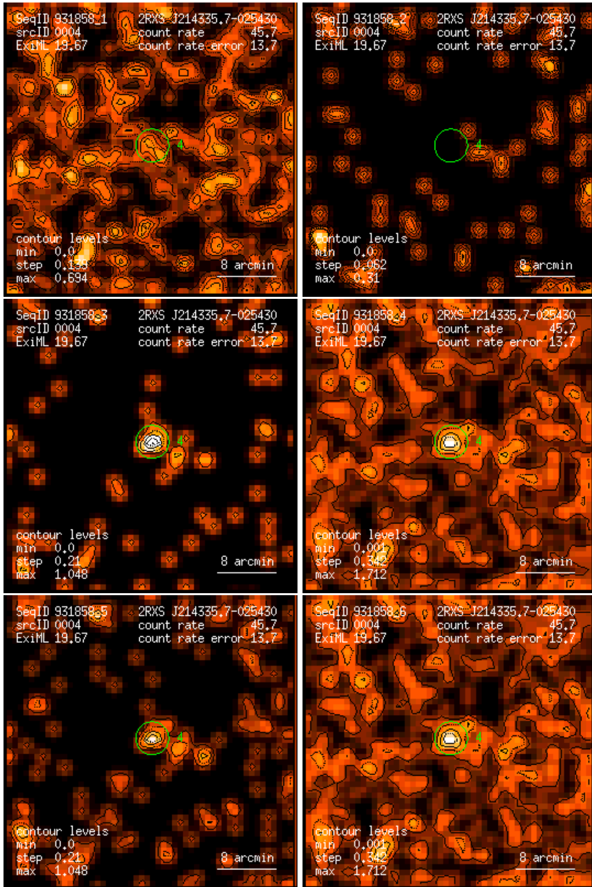
Figure 4: RASS 931858: detection 0004: band rate images, Gaussian filter: (1) PSPC channels 11 – 41, (2) 52 – 90, (3) 91 – 201, (4) 11 – 235, (5) 52 – 201, (6) 11 – 201. Broad band rates in counts/ks. Band rate contour levels in counts/ks/arcmin 2 .
