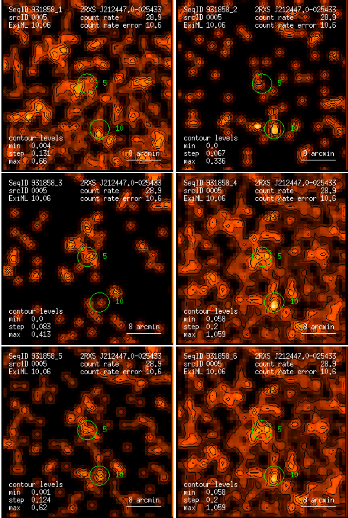
Figure 5: RASS 931858: detection 0005: band rate images, Gaussian filter: (1) PSPC channels 11 – 41, (2) 52 – 90, (3) 91 – 201, (4) 11 – 235, (5) 52 – 201, (6) 11 – 201. Broad band rates in counts/ks. Band rate contour levels in counts/ks/arcmin 2 .
