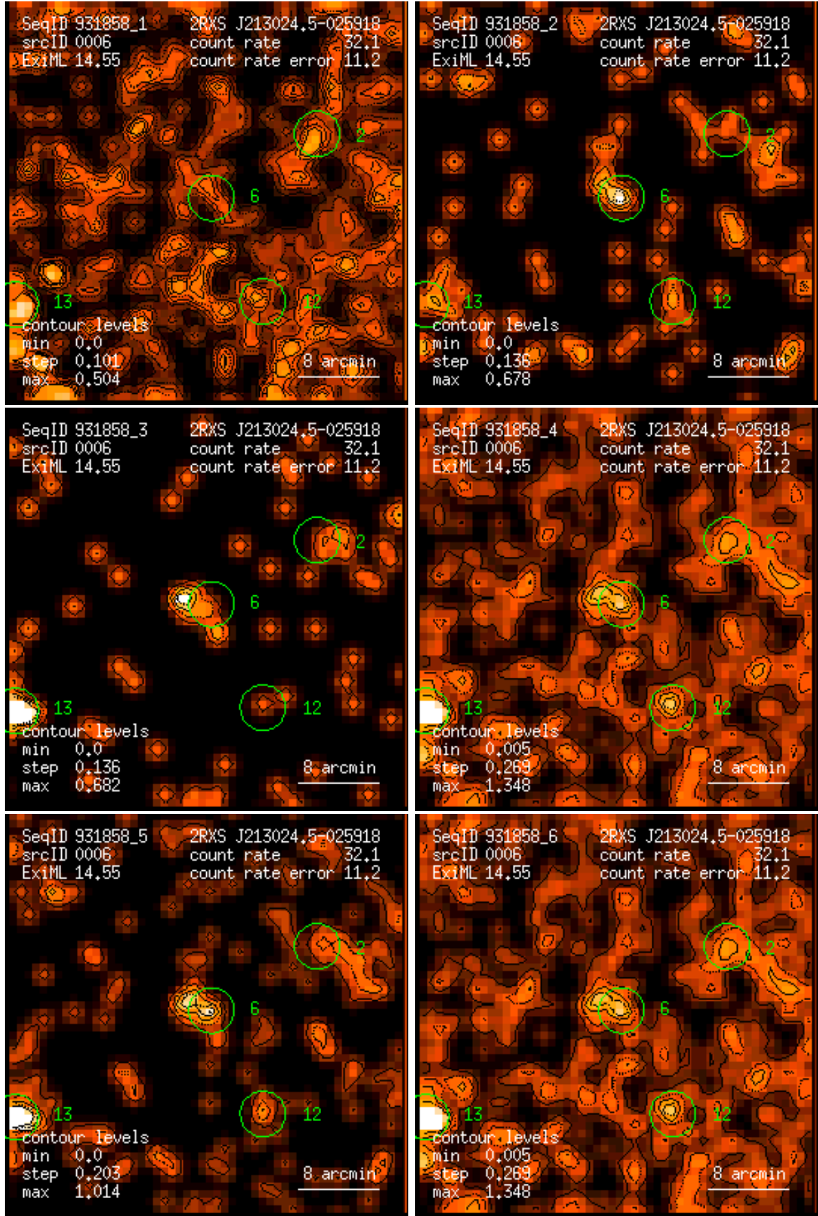
Figure 6: RASS 931858: detection 0006: band rate images, Gaussian filter: (1) PSPC channels 11 – 41, (2) 52 – 90, (3) 91 – 201, (4) 11 – 235, (5) 52 – 201, (6) 11 – 201. Broad band rates in counts/ks. Band rate contour levels in counts/ks/arcmin 2 .
