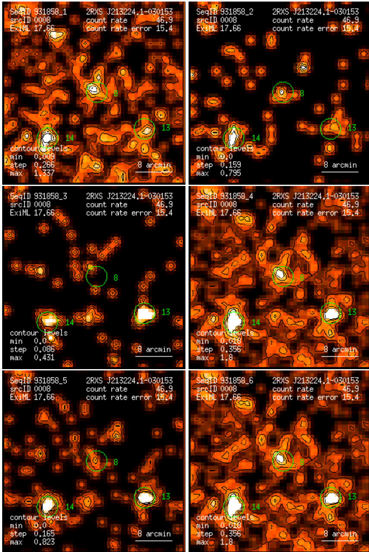
Figure 8: RASS 931858: detection 0008: band rate images, Gaussian filter: (1) PSPC channels 11 – 41, (2) 52 – 90, (3) 91 – 201, (4) 11 – 235, (5) 52 – 201, (6) 11 – 201. Broad band rates in counts/ks. Band rate contour levels in counts/ks/arcmin 2 .
