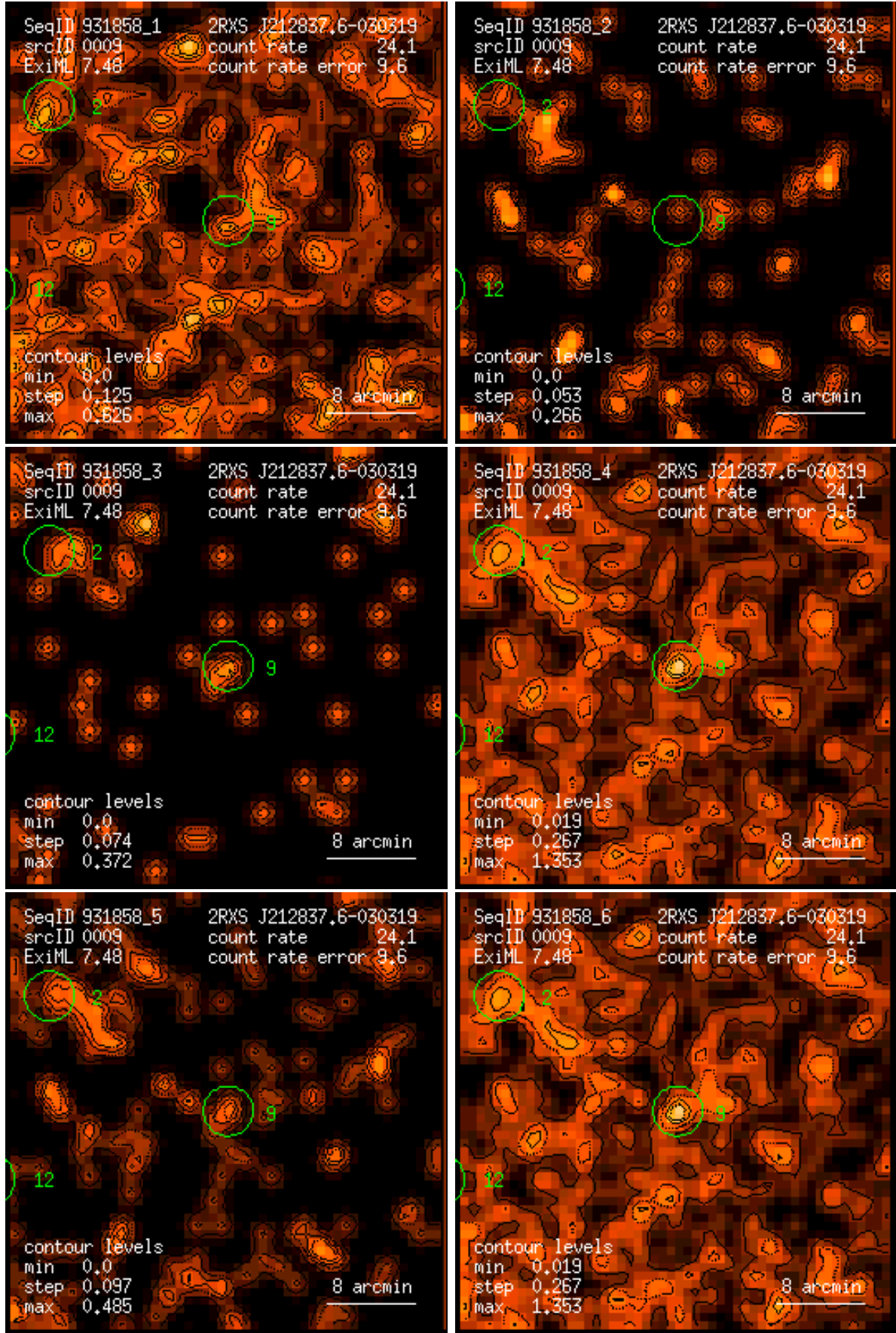
Figure 9: RASS 931858: detection 0009: band rate images, Gaussian filter: (1) PSPC channels 11 – 41, (2) 52 – 90, (3) 91 – 201, (4) 11 – 235, (5) 52 – 201, (6) 11 – 201. Broad band rates in counts/ks. Band rate contour levels in counts/ks/arcmin 2 .
