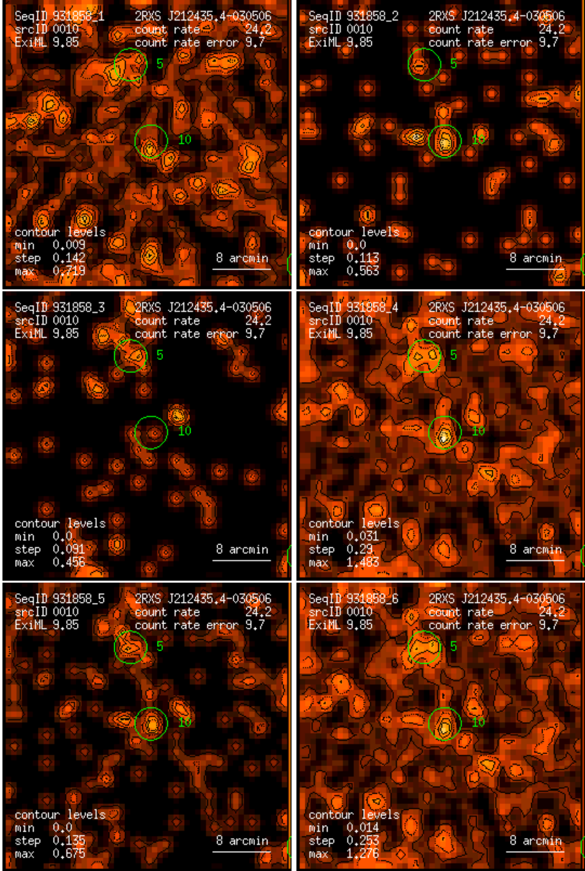
Figure 10: RASS 931858: detection 0010: band rate images, Gaussian filter: (1) PSPC channels 11 – 41, (2) 52 – 90, (3) 91 – 201, (4) 11 – 235, (5) 52 – 201, (6) 11 – 201. Broad band rates in counts/ks. Band rate contour levels in counts/ks/arcmin 2 .
