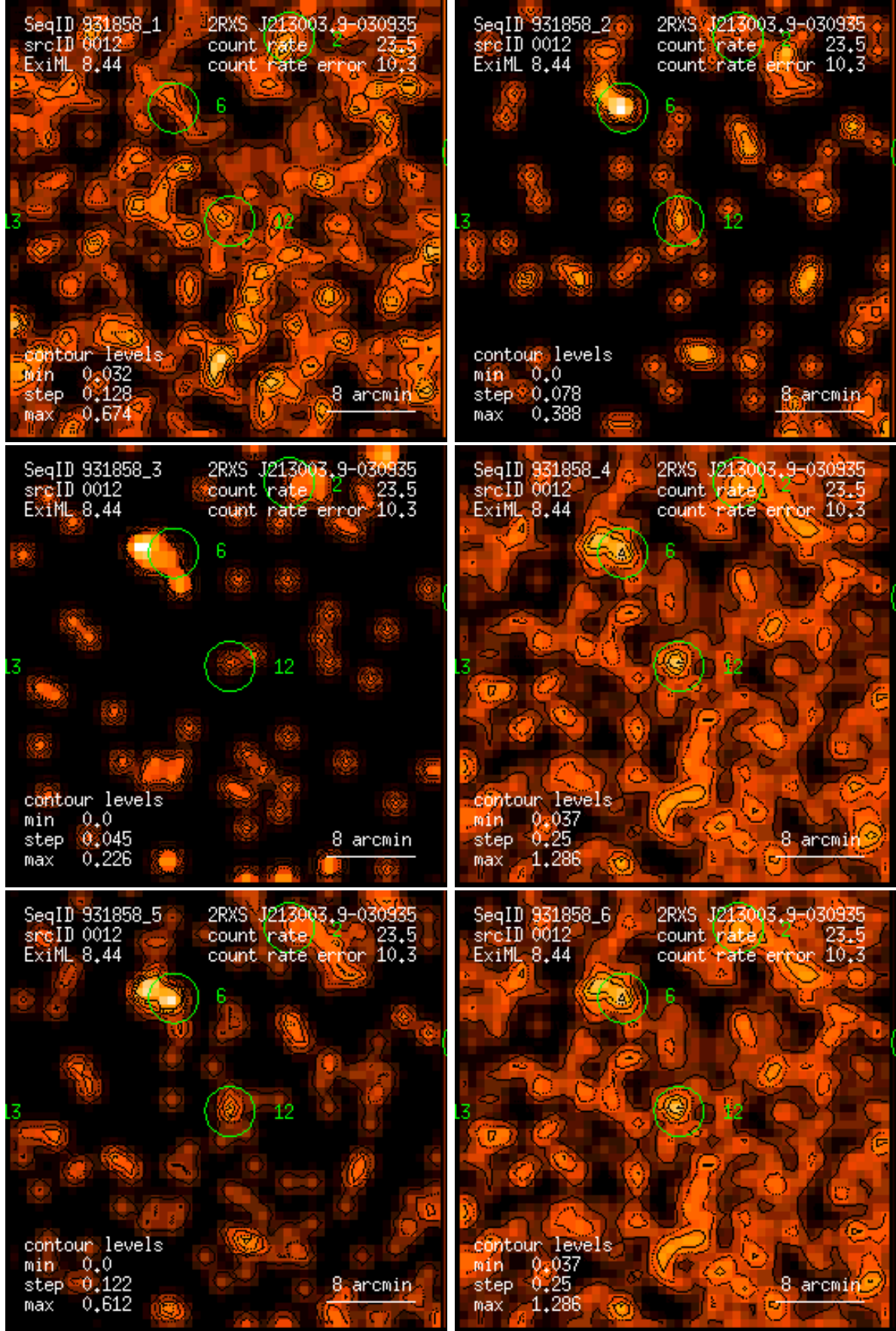
Figure 12: RASS 931858: detection 0012: band rate images, Gaussian filter: (1) PSPC channels 11 – 41, (2) 52 – 90, (3) 91 – 201, (4) 11 – 235, (5) 52 – 201, (6) 11 – 201. Broad band rates in counts/ks. Band rate contour levels in counts/ks/arcmin 2 .
