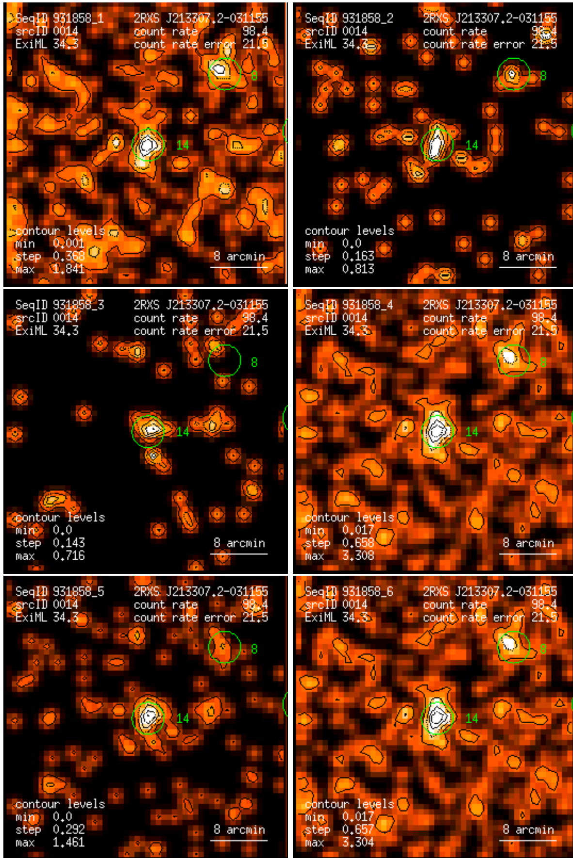
Figure 14: RASS 931858: detection 0014: band rate images, Gaussian filter: (1) PSPC channels 11 – 41, (2) 52 – 90, (3) 91 – 201, (4) 11 – 235, (5) 52 – 201, (6) 11 – 201. Broad band rates in counts/ks. Band rate contour levels in counts/ks/arcmin 2 .
