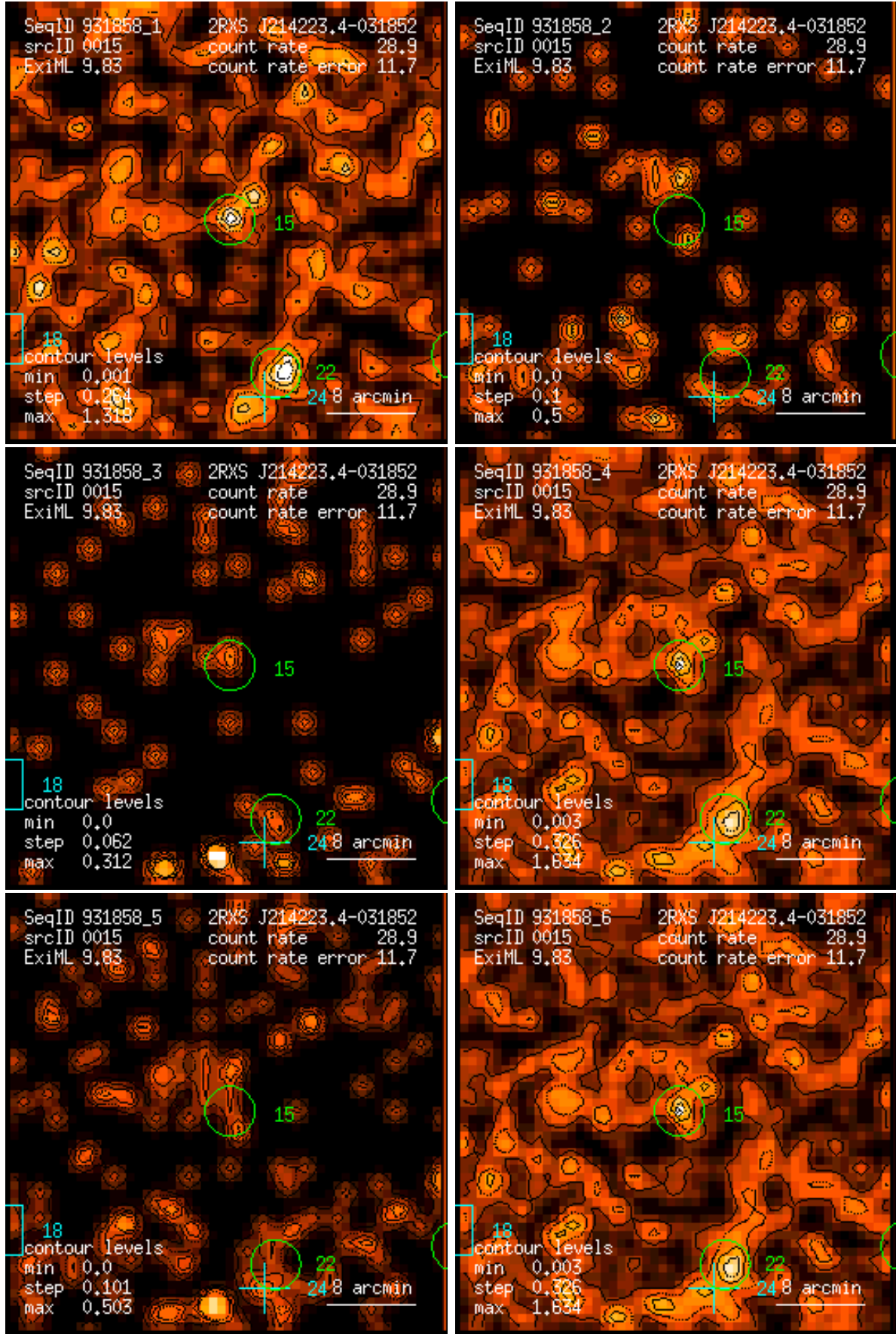
Figure 15: RASS 931858: detection 0015: band rate images, Gaussian filter: (1) PSPC channels 11 – 41, (2) 52 – 90, (3) 91 – 201, (4) 11 – 235, (5) 52 – 201, (6) 11 – 201. Broad band rates in counts/ks. Band rate contour levels in counts/ks/arcmin 2 .
