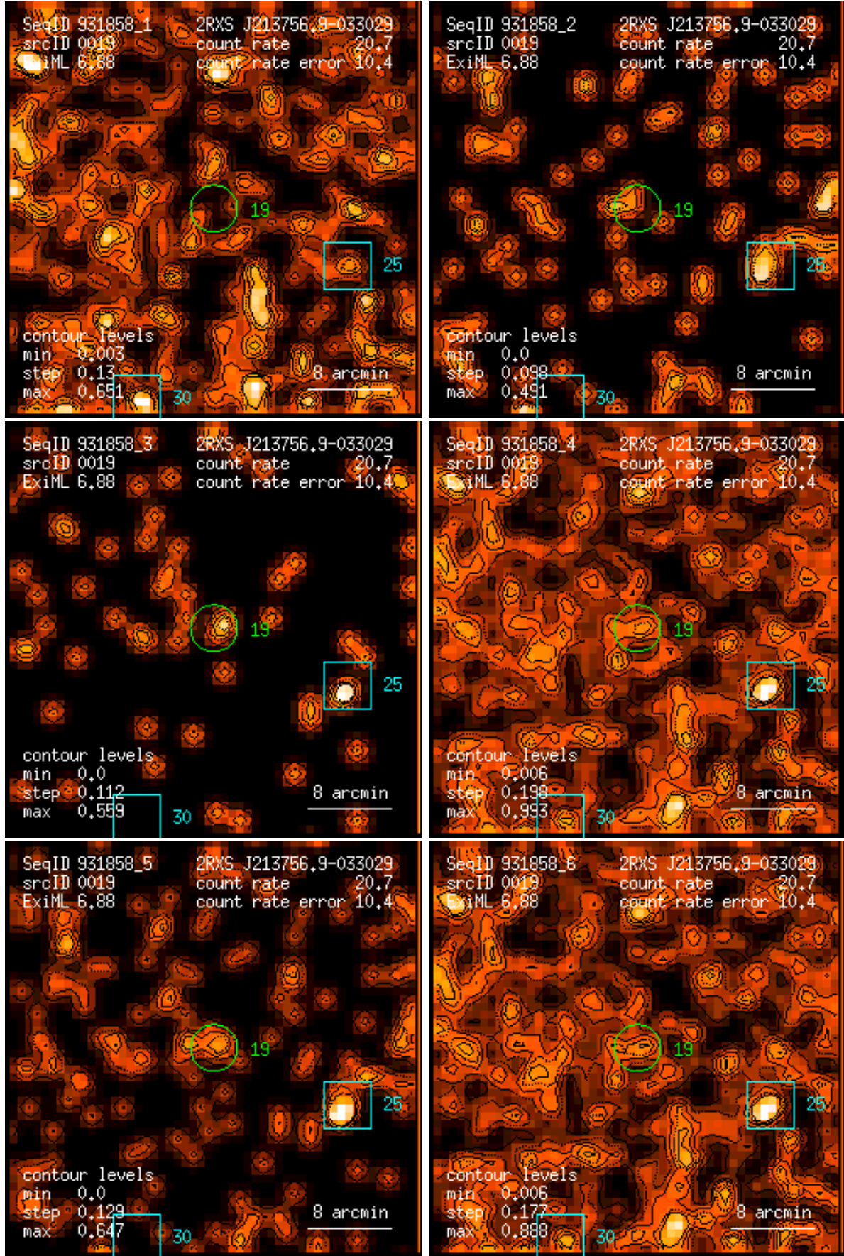
Figure 19: RASS 931858: detection 0019: band rate images, Gaussian filter: (1) PSPC channels 11 – 41, (2) 52 – 90, (3) 91 – 201, (4) 11 – 235, (5) 52 – 201, (6) 11 – 201. Broad band rates in counts/ks. Band rate contour levels in counts/ks/arcmin 2 .
