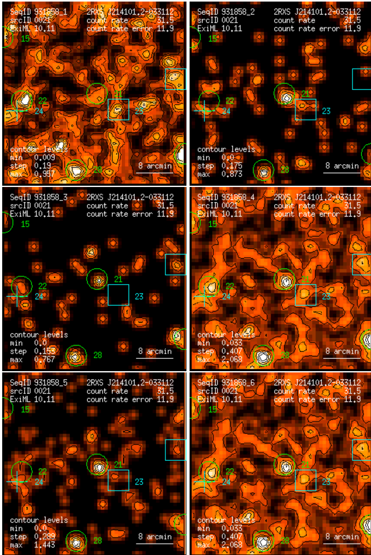
Figure 21: RASS 931858: detection 0021: band rate images, Gaussian filter: (1) PSPC channels 11 – 41, (2) 52 – 90, (3) 91 – 201, (4) 11 – 235, (5) 52 – 201, (6) 11 – 201. Broad band rates in counts/ks. Band rate contour levels in counts/ks/arcmin 2 .
