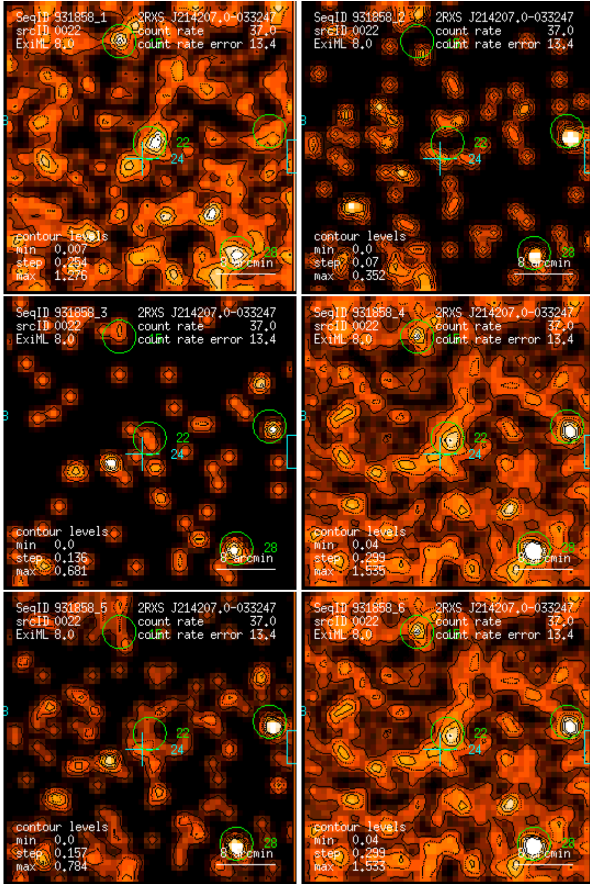
Figure 22: RASS 931858: detection 0022: band rate images, Gaussian filter: (1) PSPC channels 11 – 41, (2) 52 – 90, (3) 91 – 201, (4) 11 – 235, (5) 52 – 201, (6) 11 – 201. Broad band rates in counts/ks. Band rate contour levels in counts/ks/arcmin 2 .
