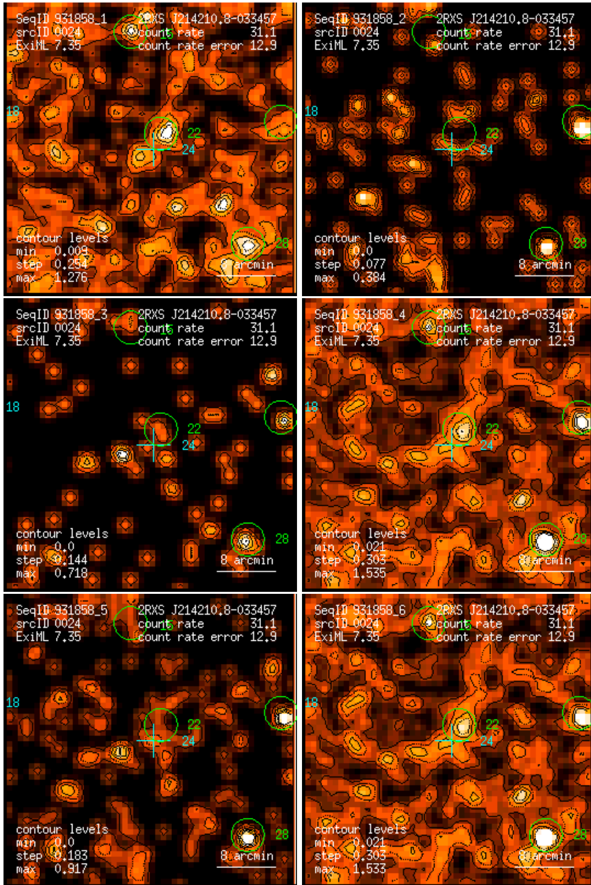
Figure 24: RASS 931858: detection 0024: band rate images, Gaussian filter: (1) PSPC channels 11 – 41, (2) 52 – 90, (3) 91 – 201, (4) 11 – 235, (5) 52 – 201, (6) 11 – 201. Broad band rates in counts/ks. Band rate contour levels in counts/ks/arcmin 2 .
