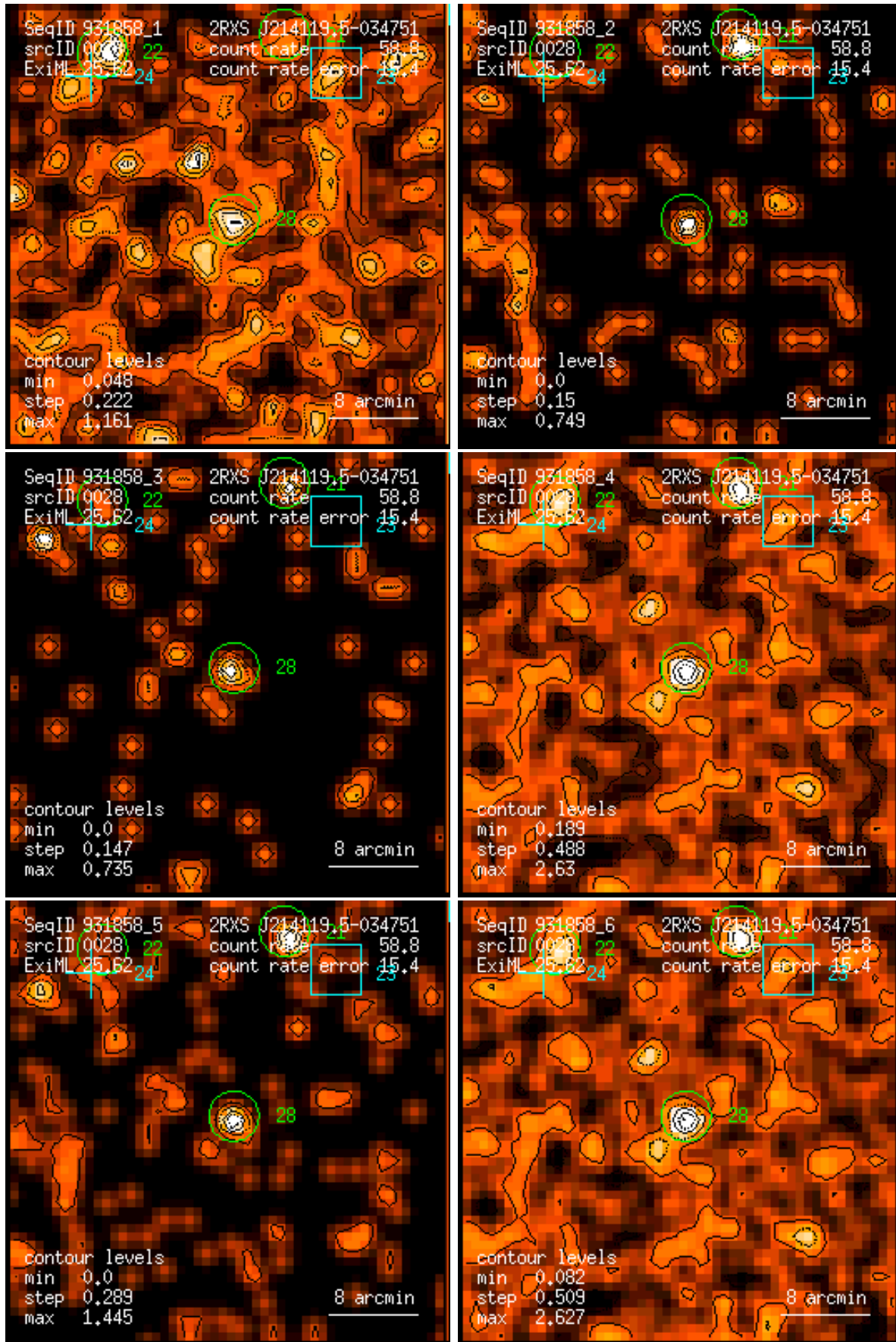
Figure 28: RASS 931858: detection 0028: band rate images, Gaussian filter: (1) PSPC channels 11 – 41, (2) 52 – 90, (3) 91 – 201, (4) 11 – 235, (5) 52 – 201, (6) 11 – 201. Broad band rates in counts/ks. Band rate contour levels in counts/ks/arcmin 2 .
