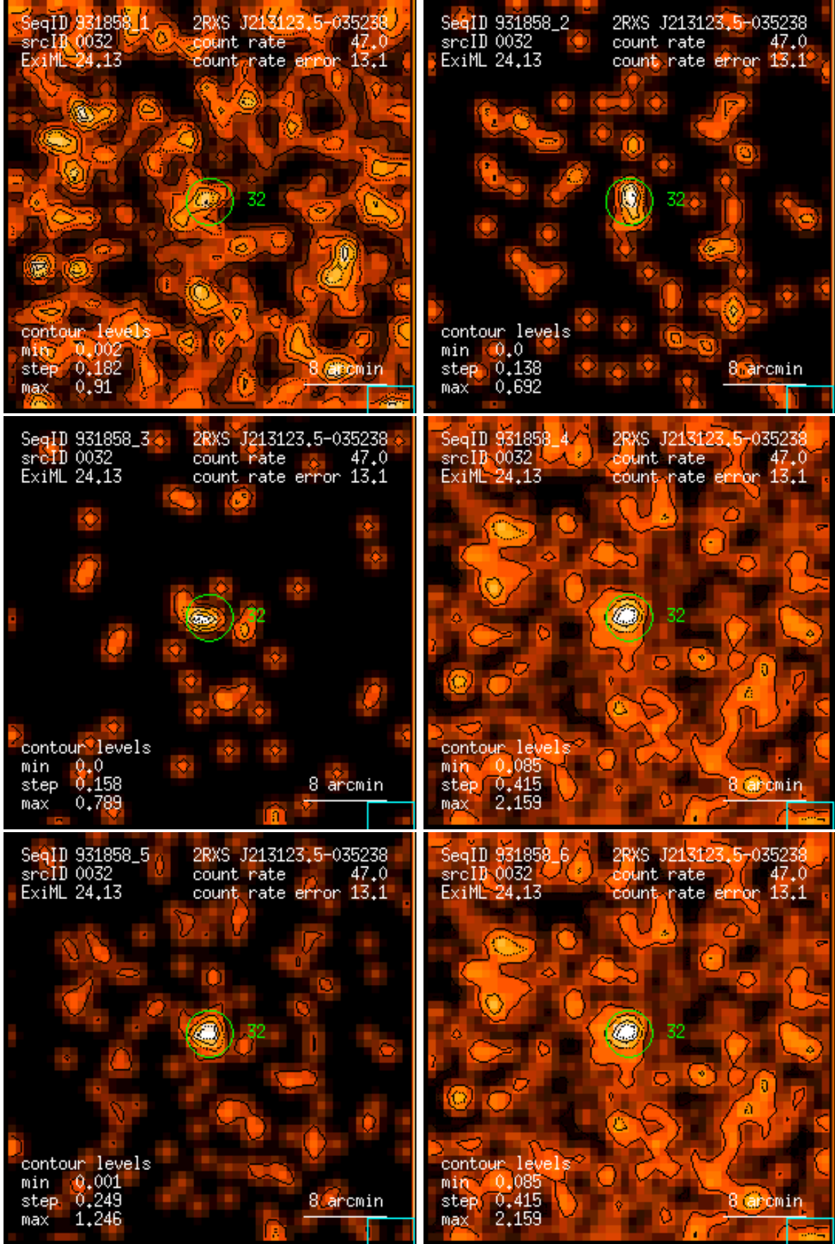
Figure 32: RASS 931858: detection 0032: band rate images, Gaussian filter: (1) PSPC channels 11 – 41, (2) 52 – 90, (3) 91 – 201, (4) 11 – 235, (5) 52 – 201, (6) 11 – 201. Broad band rates in counts/ks. Band rate contour levels in counts/ks/arcmin 2 .
