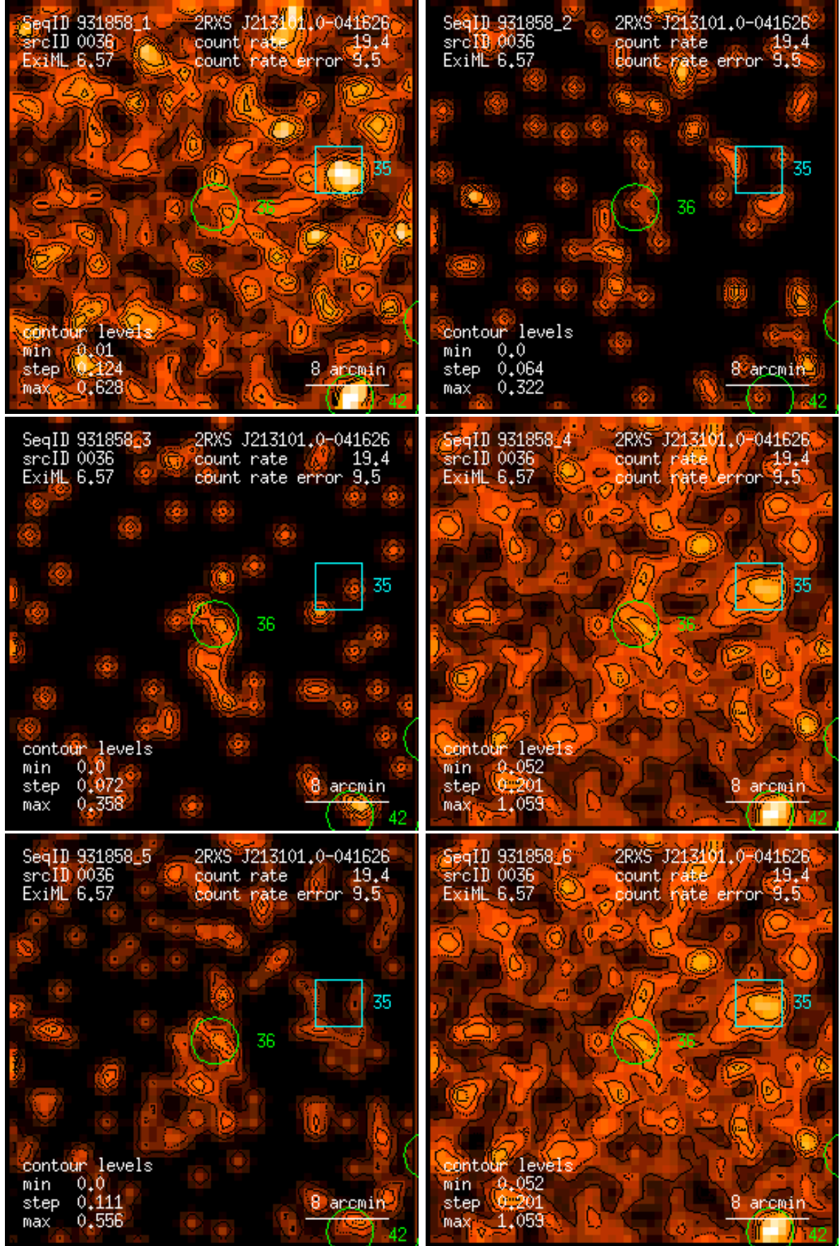
Figure 36: RASS 931858: detection 0036: band rate images, Gaussian filter: (1) PSPC channels 11 – 41, (2) 52 – 90, (3) 91 – 201, (4) 11 – 235, (5) 52 – 201, (6) 11 – 201. Broad band rates in counts/ks. Band rate contour levels in counts/ks/arcmin 2 .
