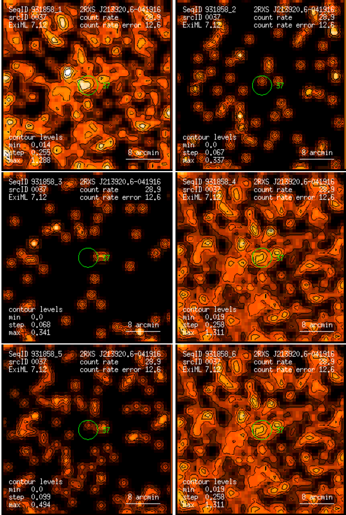
Figure 37: RASS 931858: detection 0037: band rate images, Gaussian filter: (1) PSPC channels 11 – 41, (2) 52 – 90, (3) 91 – 201, (4) 11 – 235, (5) 52 – 201, (6) 11 – 201. Broad band rates in counts/ks. Band rate contour levels in counts/ks/arcmin 2 .
