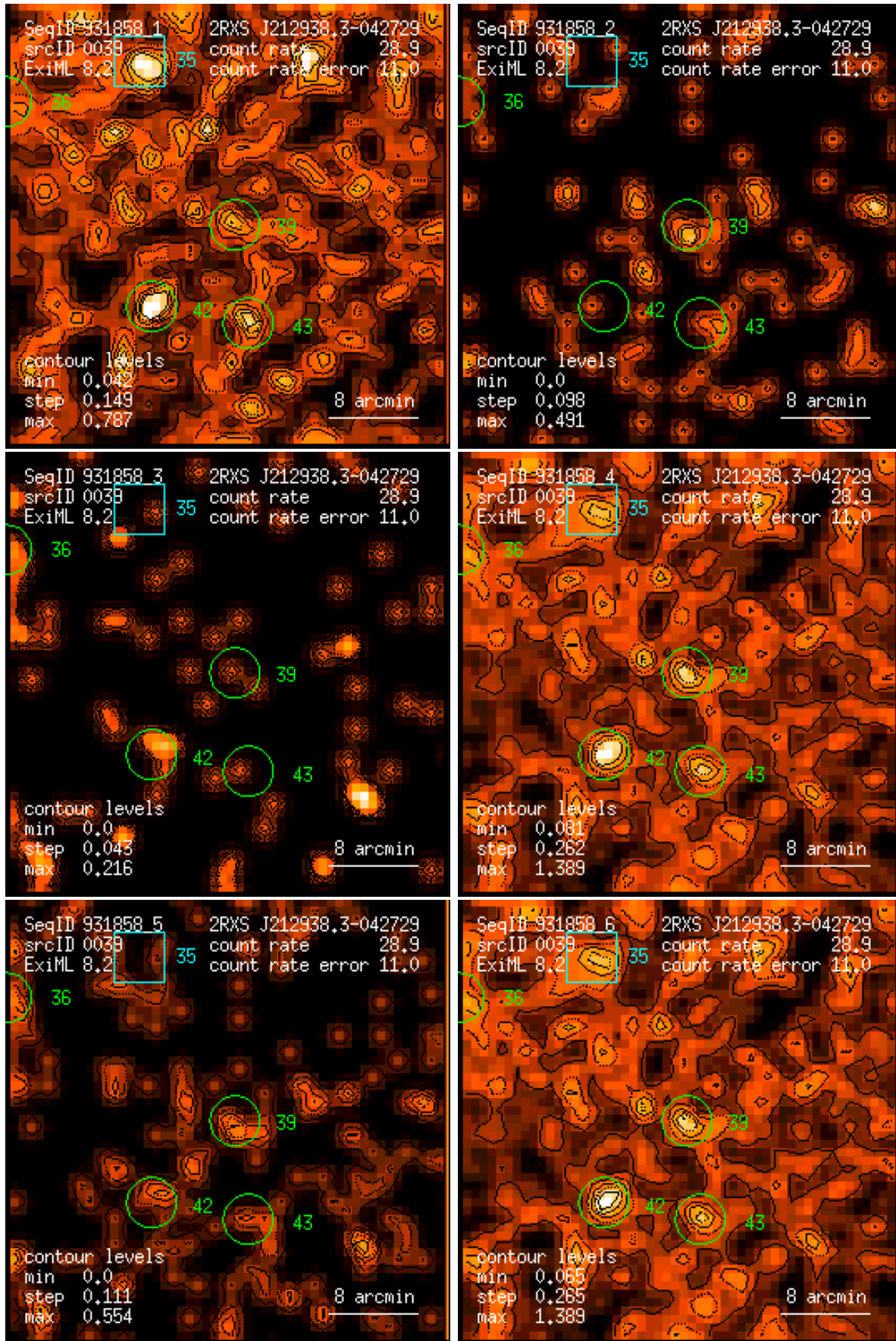
Figure 39: RASS 931858: detection 0039: band rate images, Gaussian filter: (1) PSPC channels 11 – 41, (2) 52 – 90, (3) 91 – 201, (4) 11 – 235, (5) 52 – 201, (6) 11 – 201. Broad band rates in counts/ks. Band rate contour levels in counts/ks/arcmin 2 .
