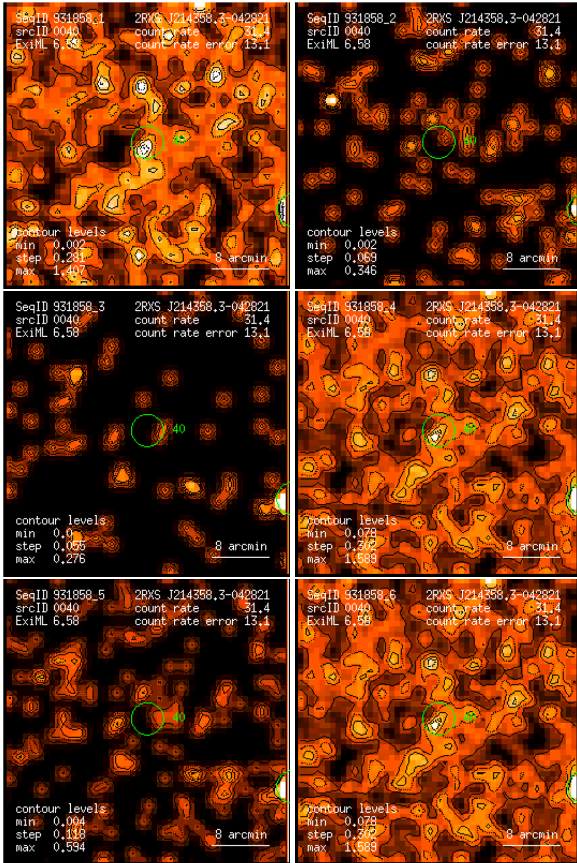
Figure 40: RASS 931858: detection 0040: band rate images, Gaussian filter: (1) PSPC channels 11 – 41, (2) 52 – 90, (3) 91 – 201, (4) 11 – 235, (5) 52 – 201, (6) 11 – 201. Broad band rates in counts/ks. Band rate contour levels in counts/ks/arcmin 2 .
