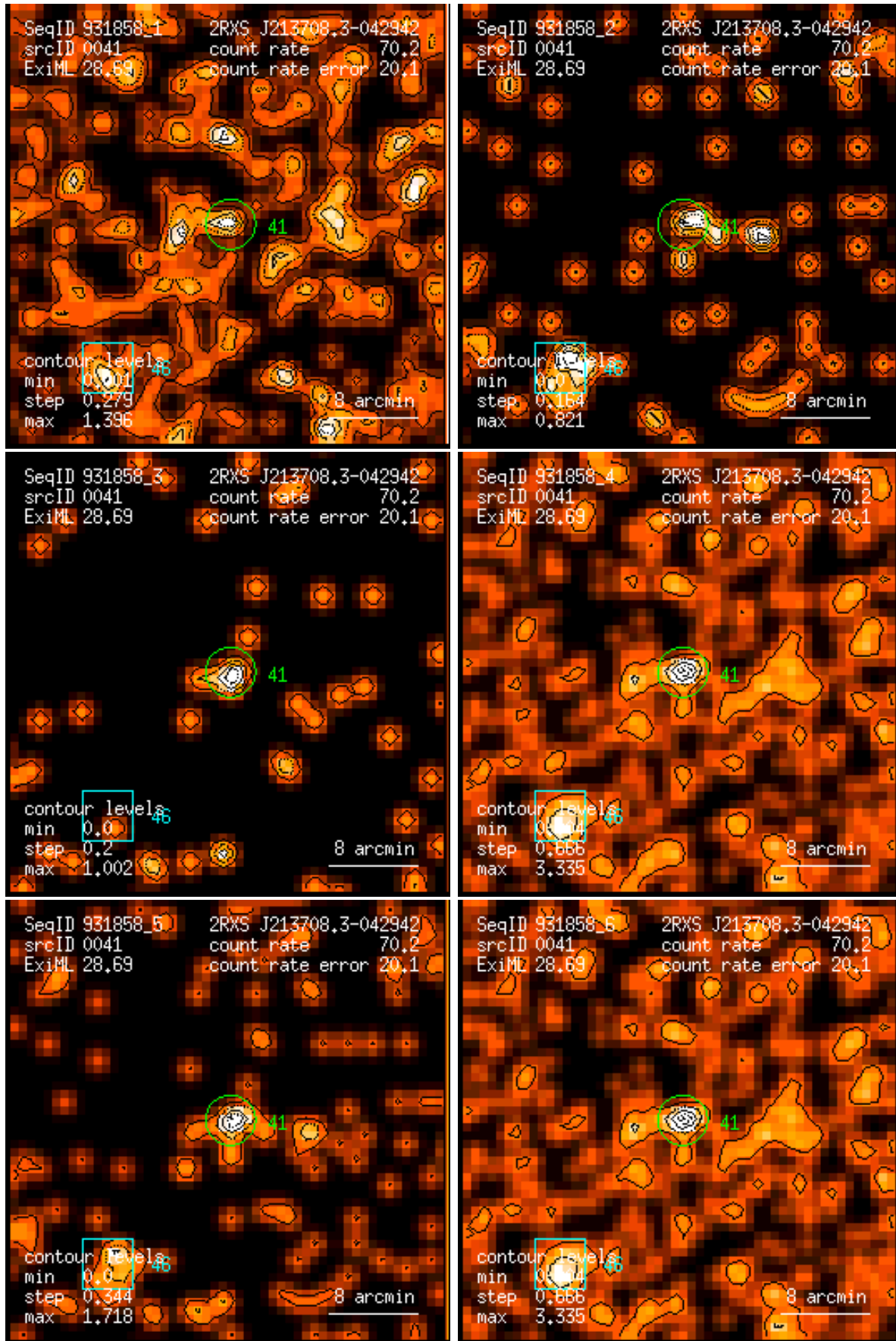
Figure 41: RASS 931858: detection 0041: band rate images, Gaussian filter: (1) PSPC channels 11 – 41, (2) 52 – 90, (3) 91 – 201, (4) 11 – 235, (5) 52 – 201, (6) 11 – 201. Broad band rates in counts/ks. Band rate contour levels in counts/ks/arcmin 2 .
