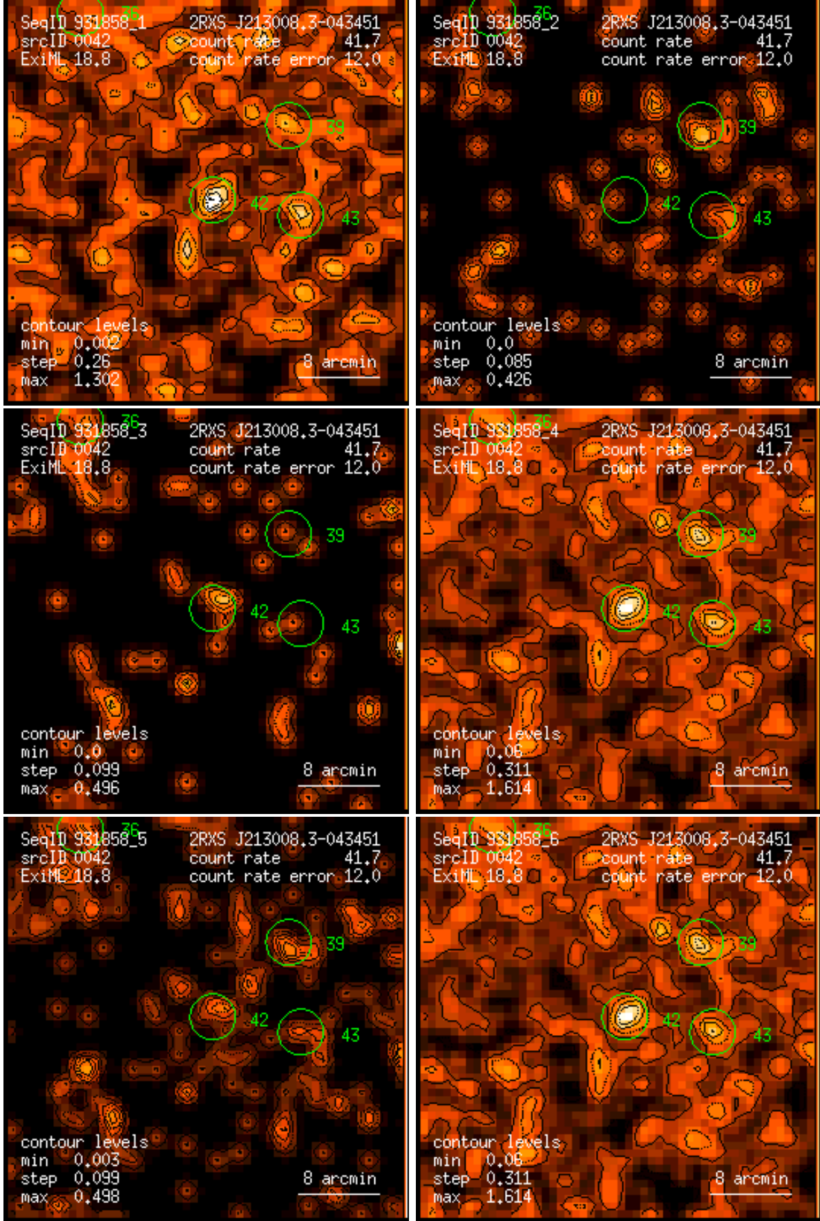
Figure 42: RASS 931858: detection 0042: band rate images, Gaussian filter: (1) PSPC channels 11 – 41, (2) 52 – 90, (3) 91 – 201, (4) 11 – 235, (5) 52 – 201, (6) 11 – 201. Broad band rates in counts/ks. Band rate contour levels in counts/ks/arcmin 2 .
