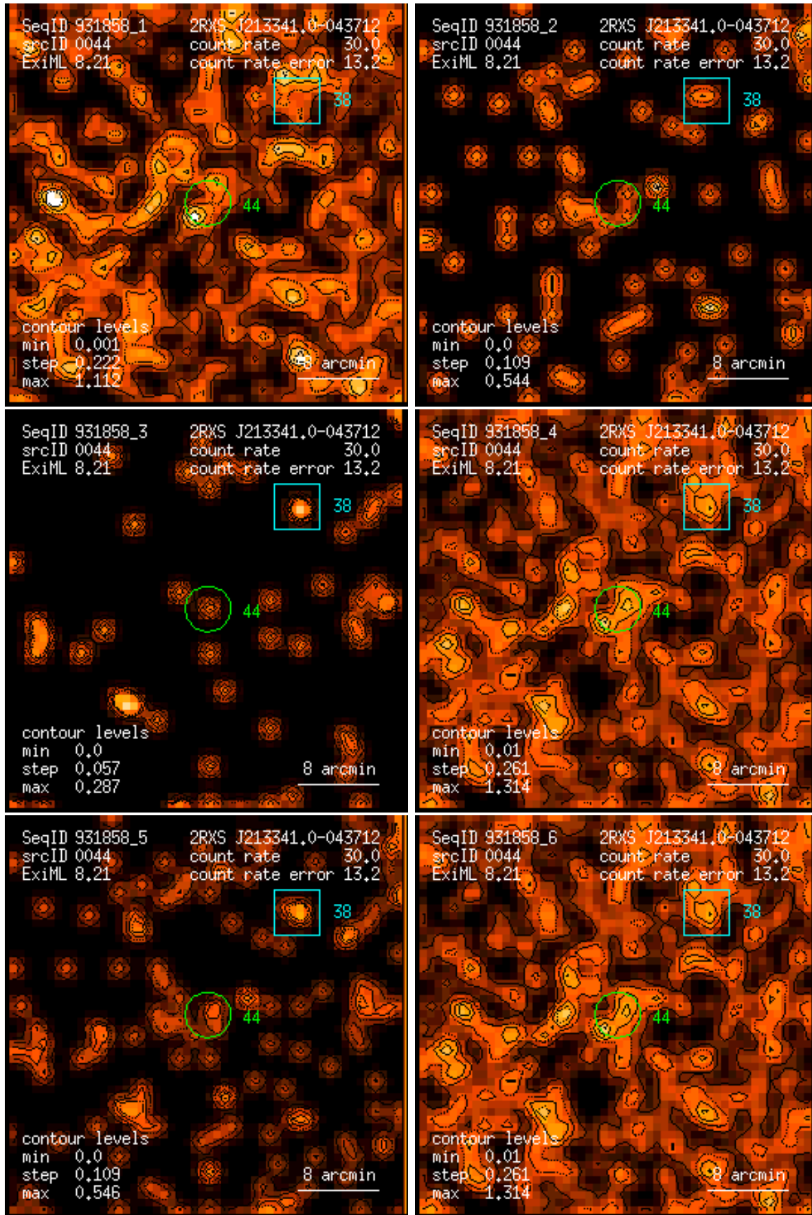
Figure 44: RASS 931858: detection 0044: band rate images, Gaussian filter: (1) PSPC channels 11 – 41, (2) 52 – 90, (3) 91 – 201, (4) 11 – 235, (5) 52 – 201, (6) 11 – 201. Broad band rates in counts/ks. Band rate contour levels in counts/ks/arcmin 2 .
