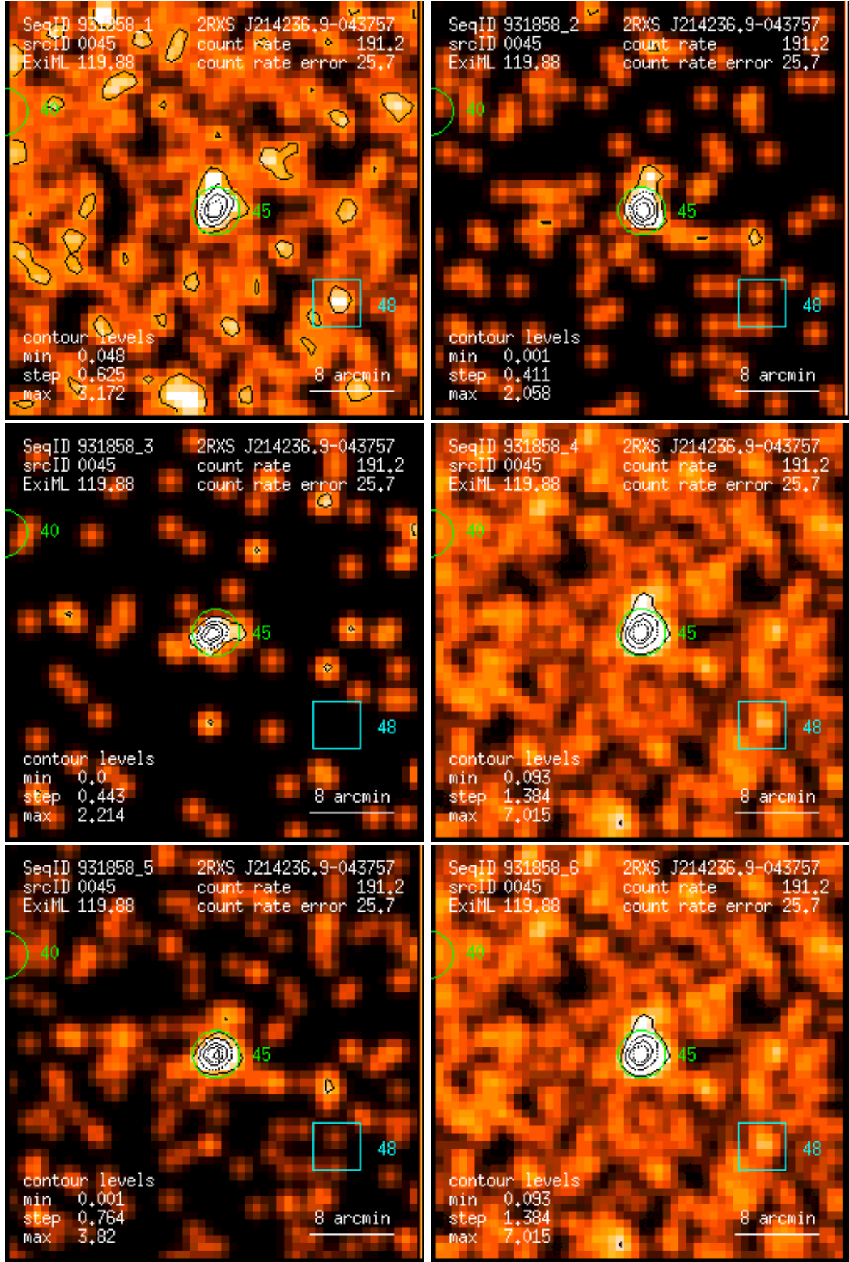
Figure 45: RASS 931858: detection 0045: band rate images, Gaussian filter: (1) PSPC channels 11 – 41, (2) 52 – 90, (3) 91 – 201, (4) 11 – 235, (5) 52 – 201, (6) 11 – 201. Broad band rates in counts/ks. Band rate contour levels in counts/ks/arcmin 2 .
